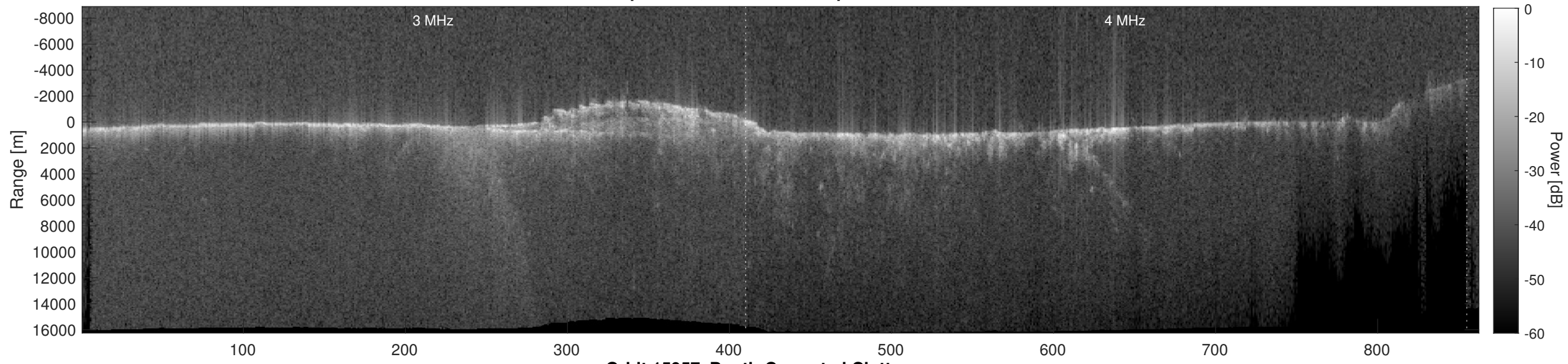
Orbit 15957, Depth-Corrected Cluttergram
