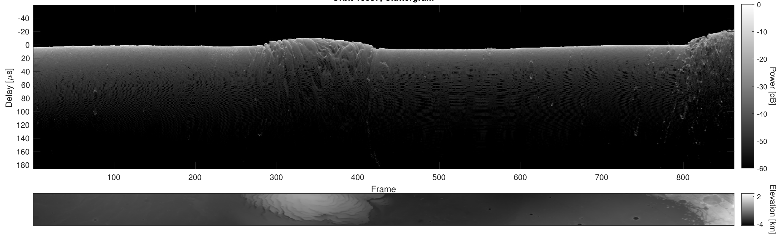
Orbit 15957, Cluttergram
