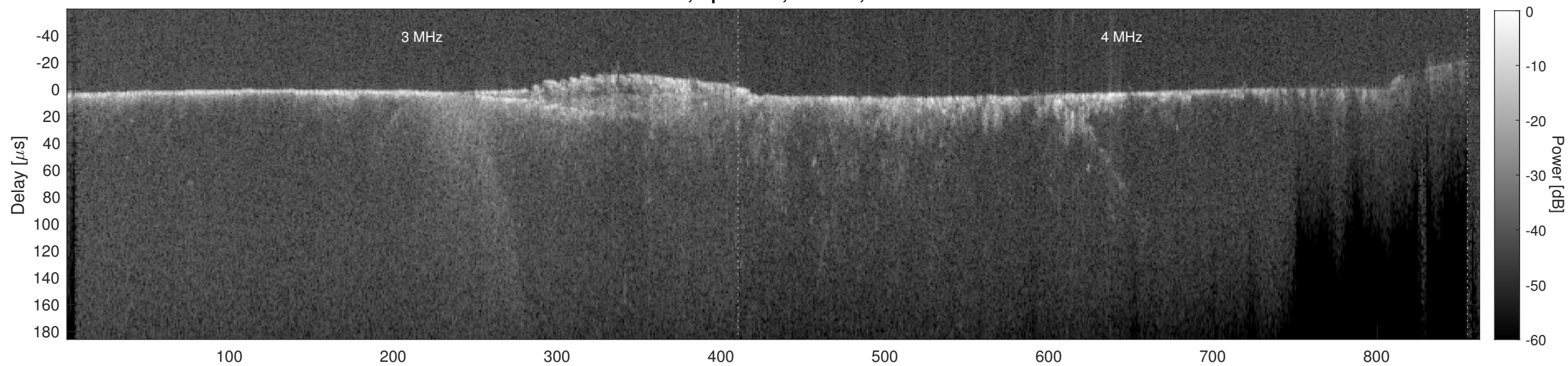
Orbit 15957, Cluttergram
