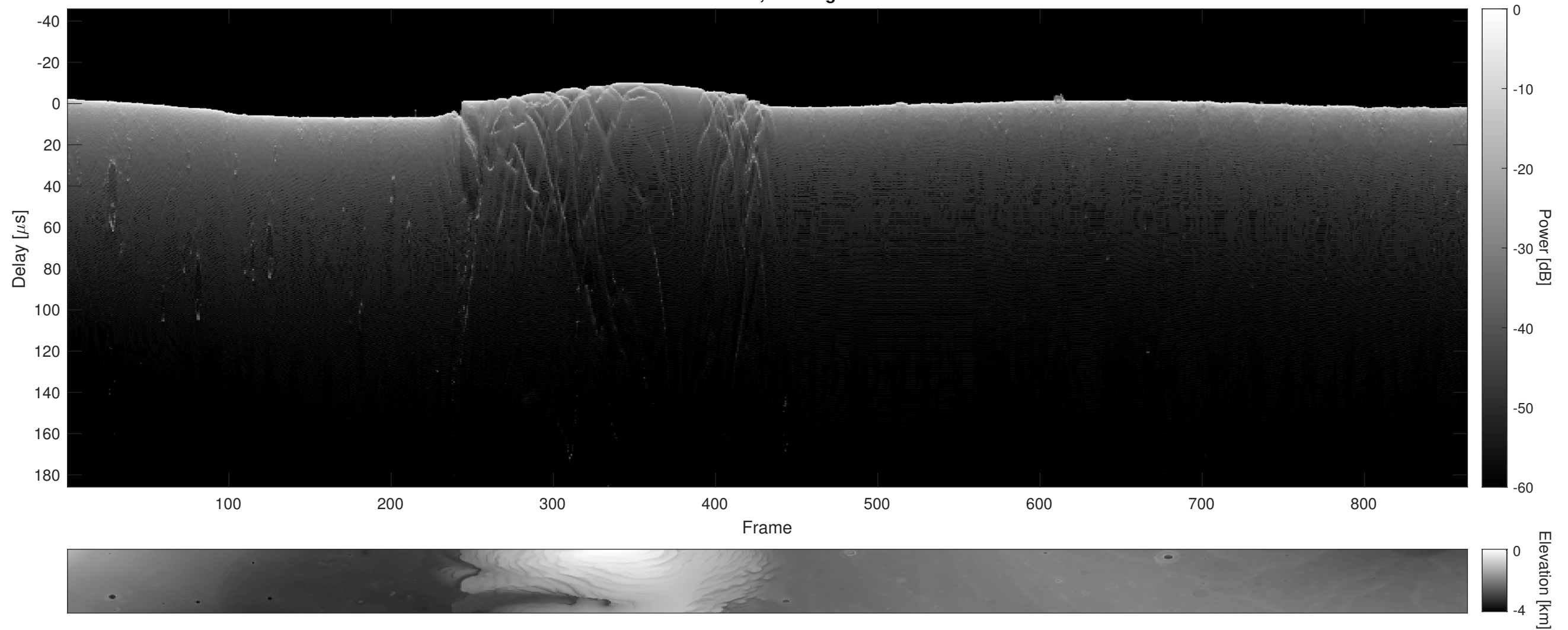
Orbit 15959, Cluttergram
