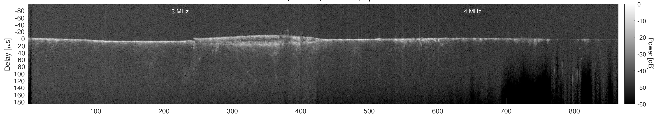
Orbit 15959, Cluttergram
