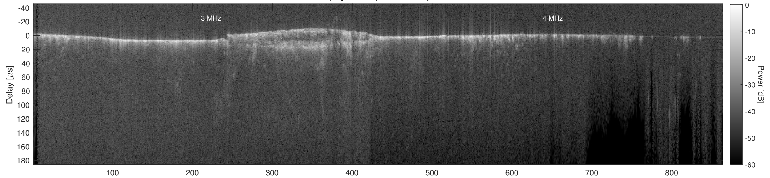
Orbit 15959, Cluttergram
