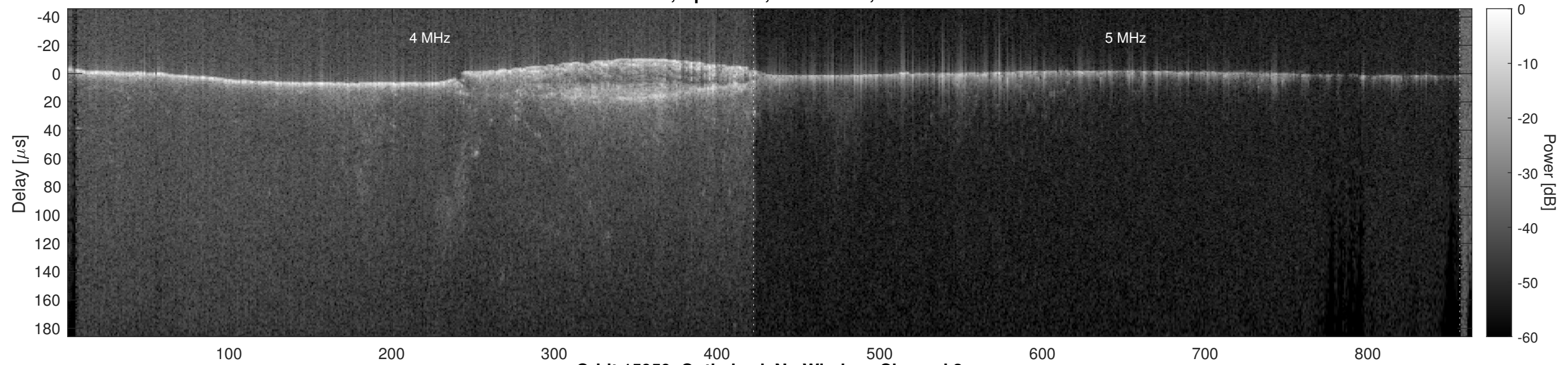
Orbit 15959, Optimized, No Window, Channel 2
