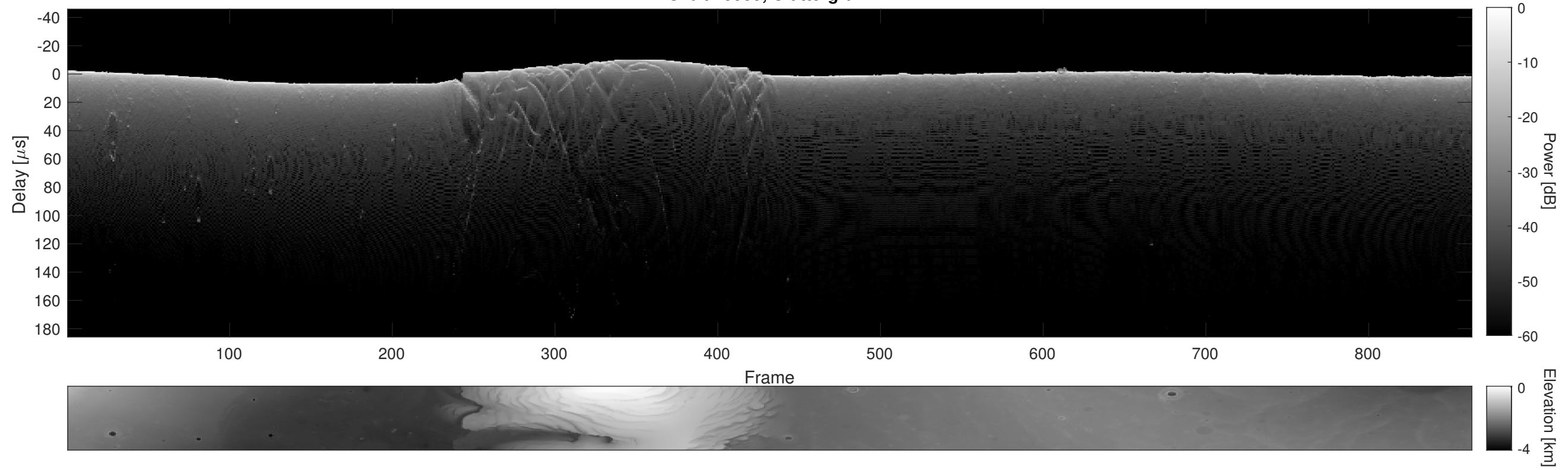
Orbit 15959, Cluttergram
