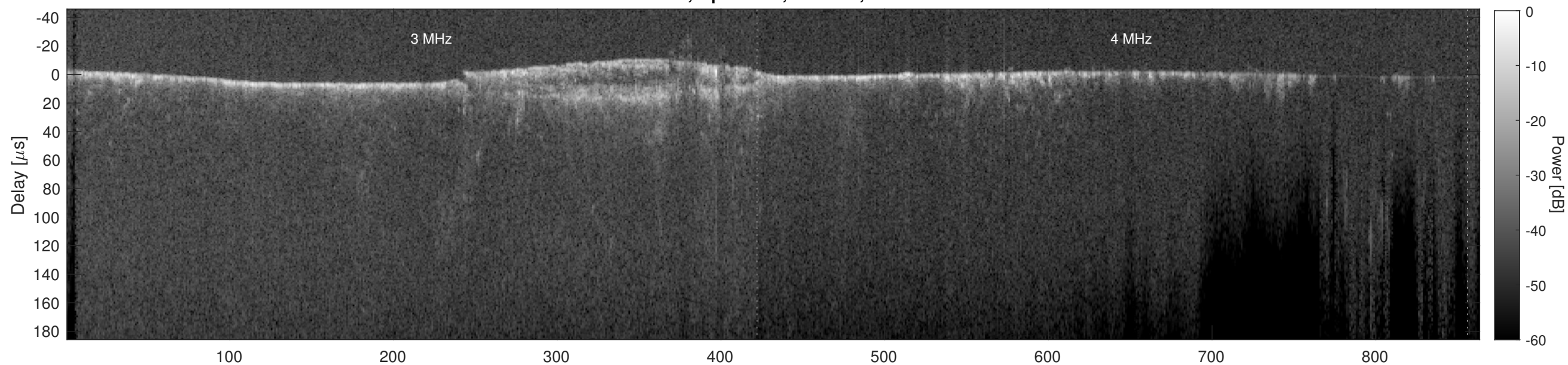
Orbit 15959, Cluttergram
