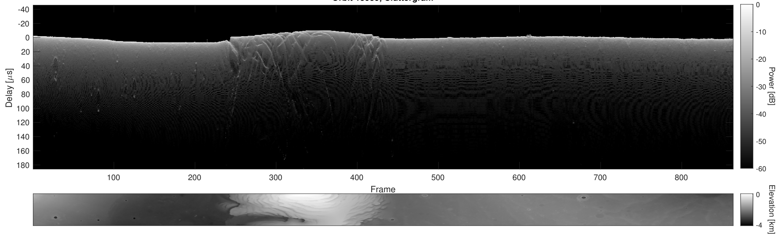
Orbit 15959, Cluttergram
