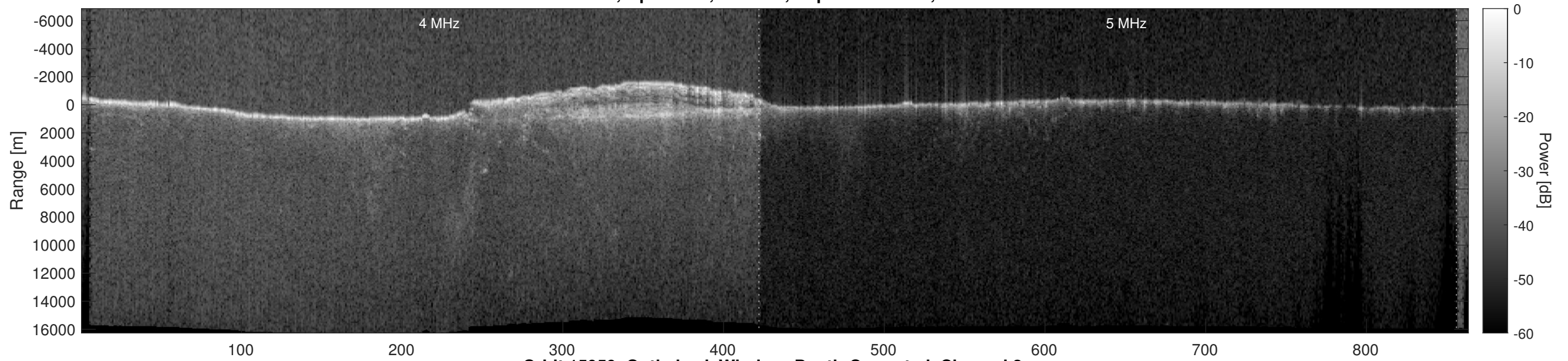
Orbit 15959, Optimized, Window, Depth-Corrected, Channel 2
