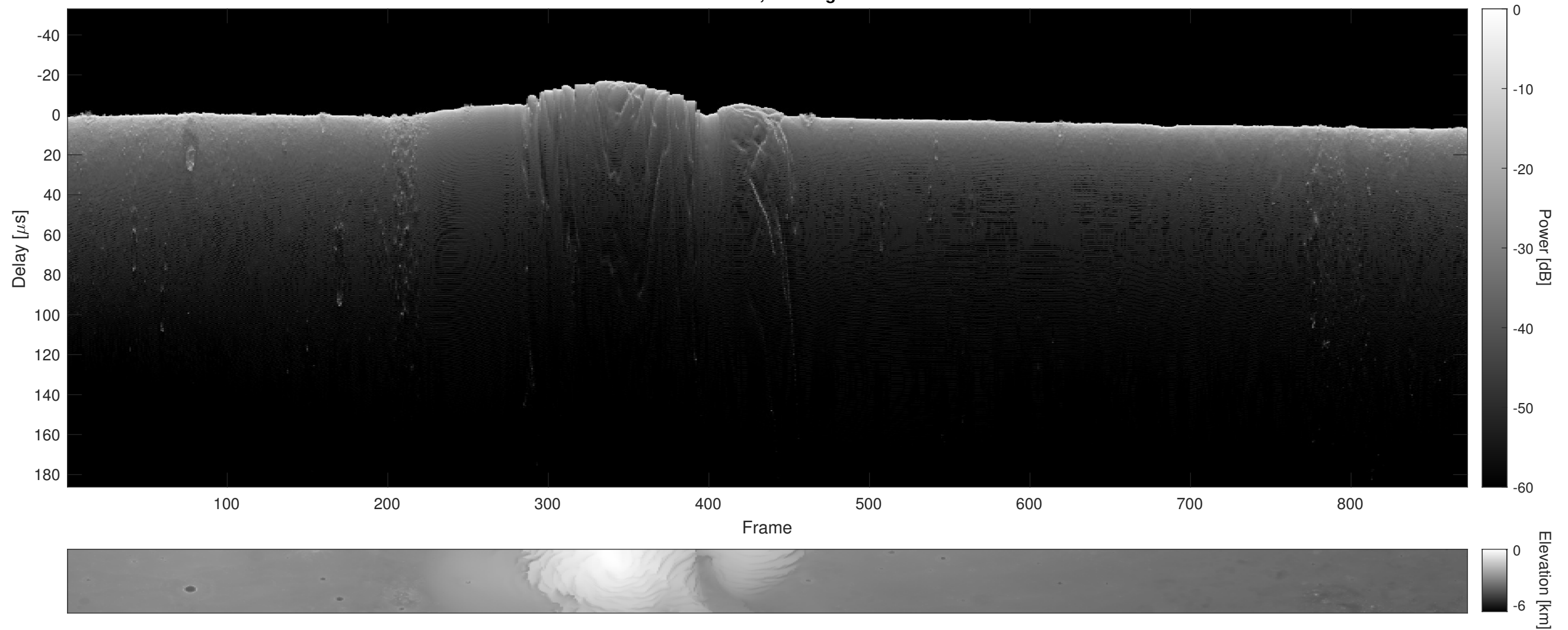
Orbit 15960, Cluttergram
