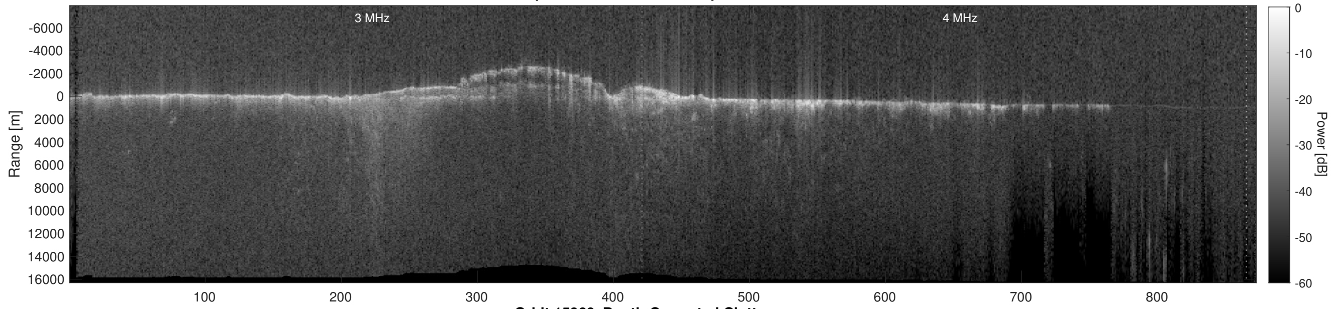
Orbit 15960, Depth-Corrected Cluttergram
