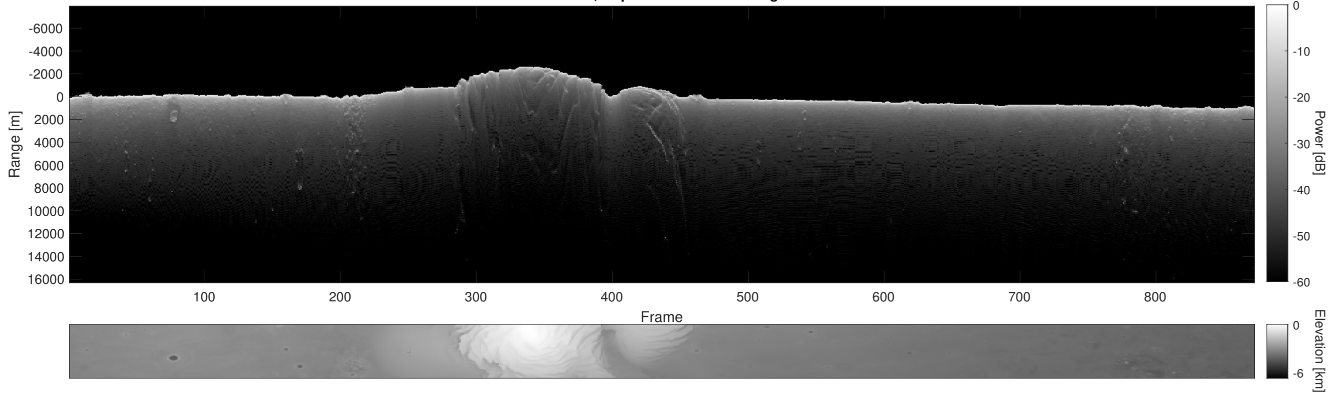
Orbit 15960, Depth-Corrected Cluttergram
