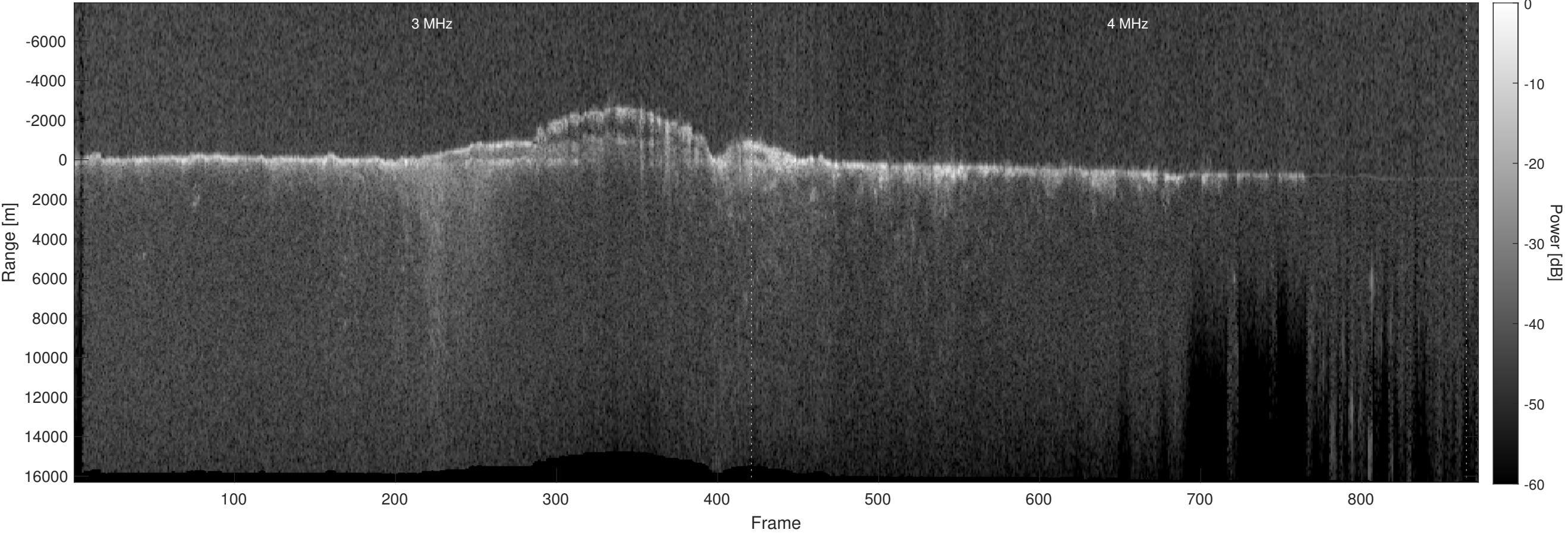
Orbit 15960, Optimized, Window, Depth-Corrected, Channel 2
