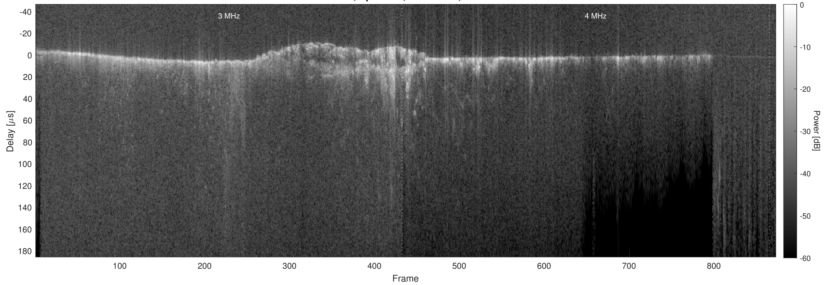
Orbit 15963, Optimized, No Window, Channel 2
