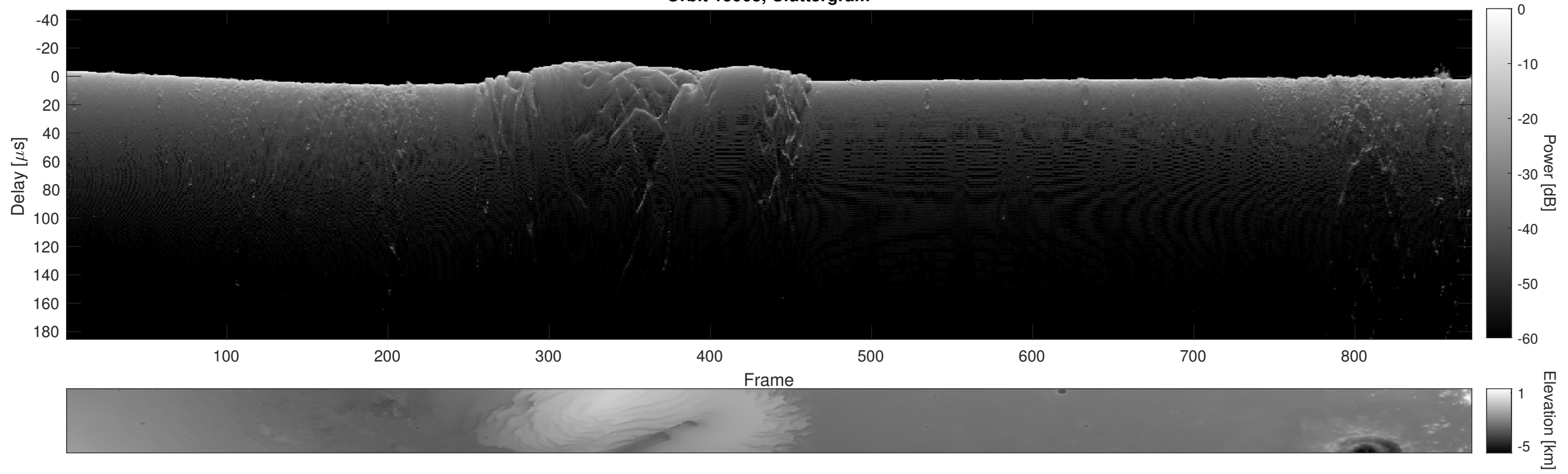
Orbit 15963, Cluttergram
