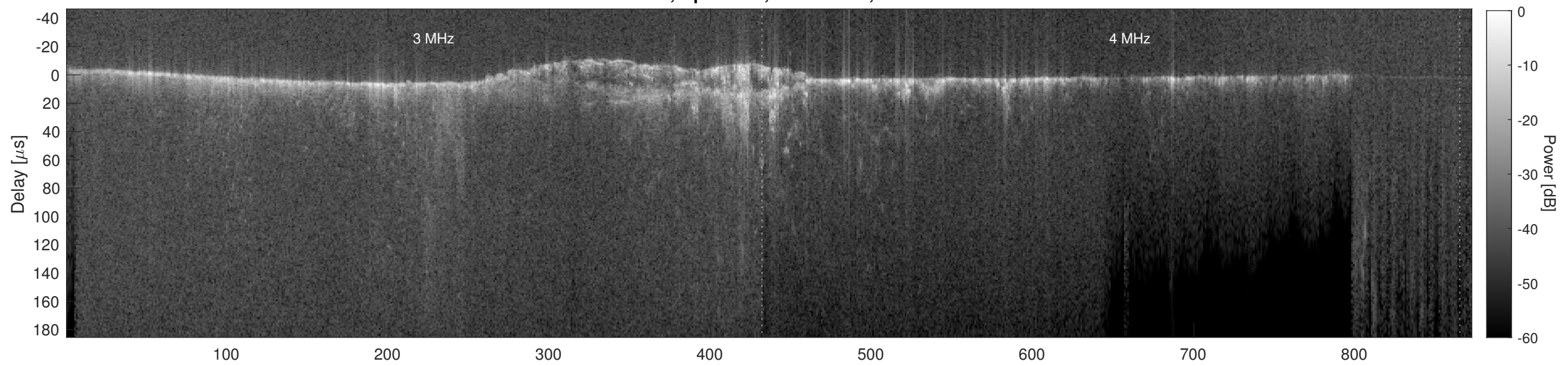
Orbit 15963, Cluttergram
