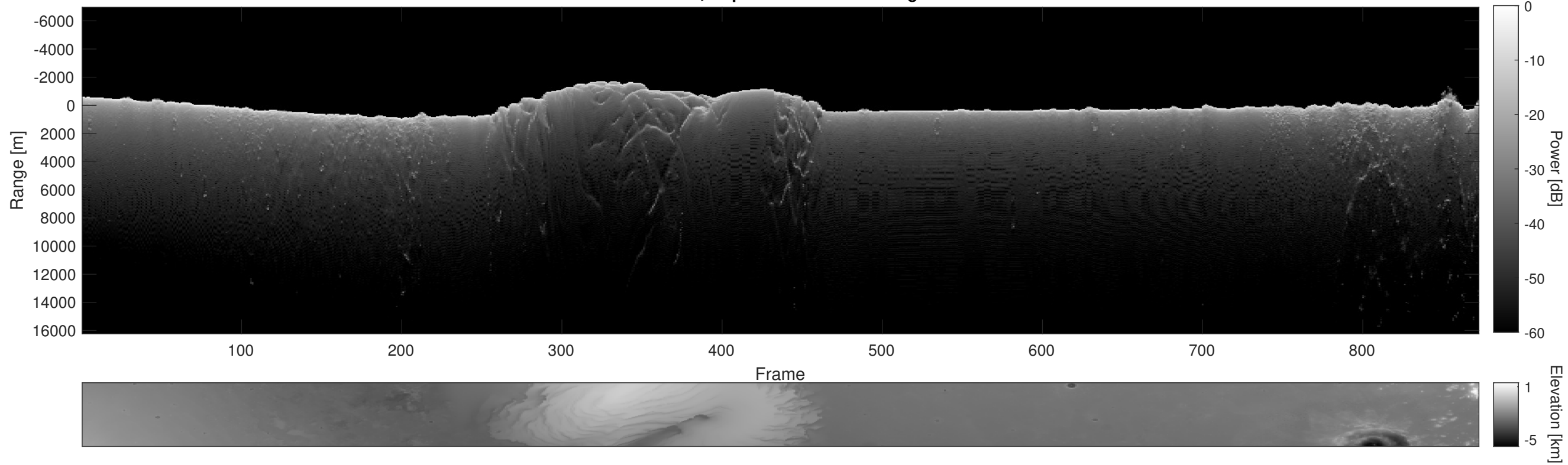
Orbit 15963, Depth-Corrected Cluttergram
