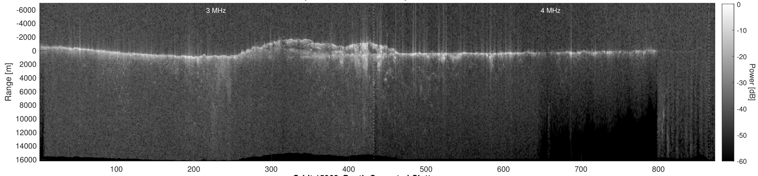
Orbit 15963, Depth-Corrected Cluttergram
