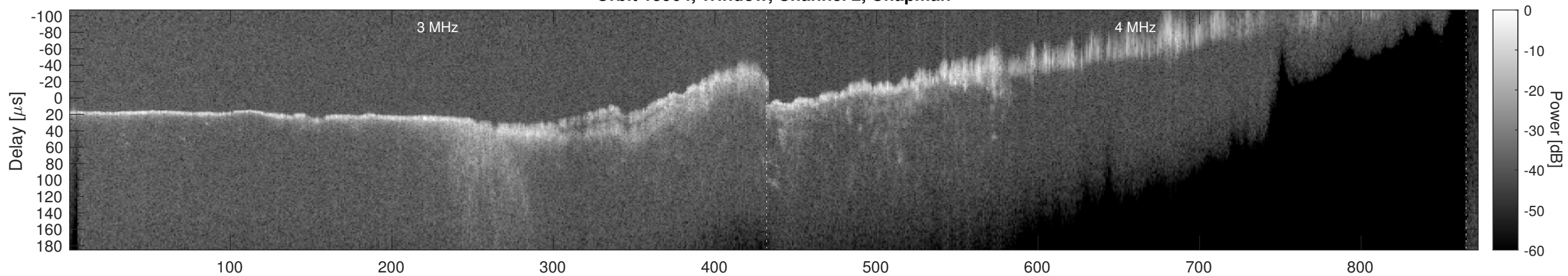
Orbit 15964, Window, Channel 2, Optimized
