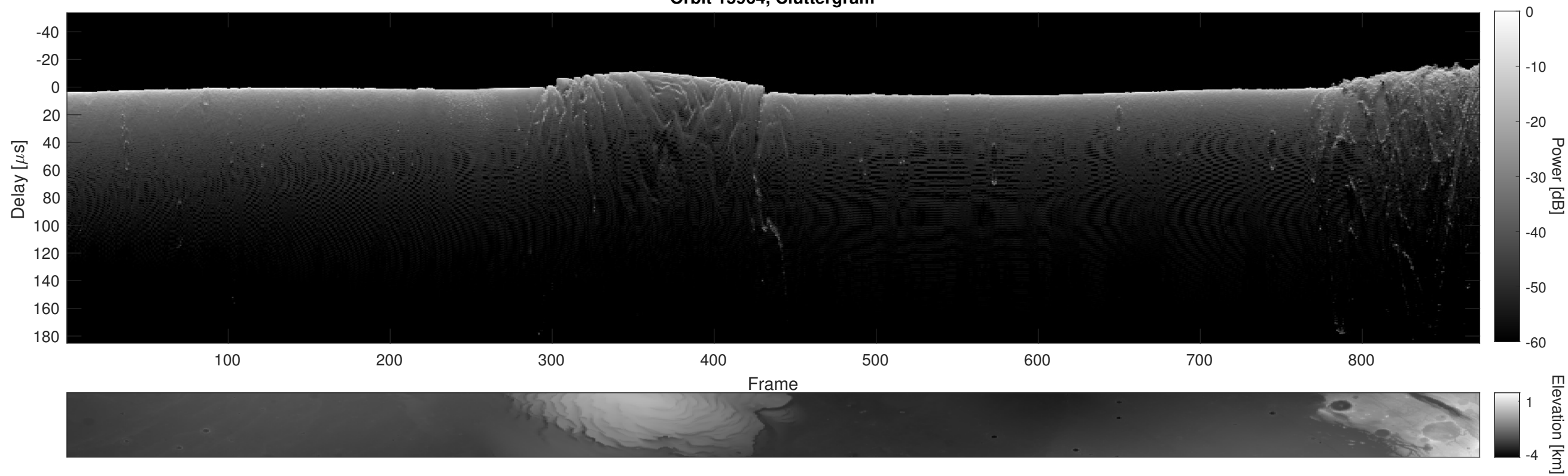
Orbit 15964, Cluttergram
