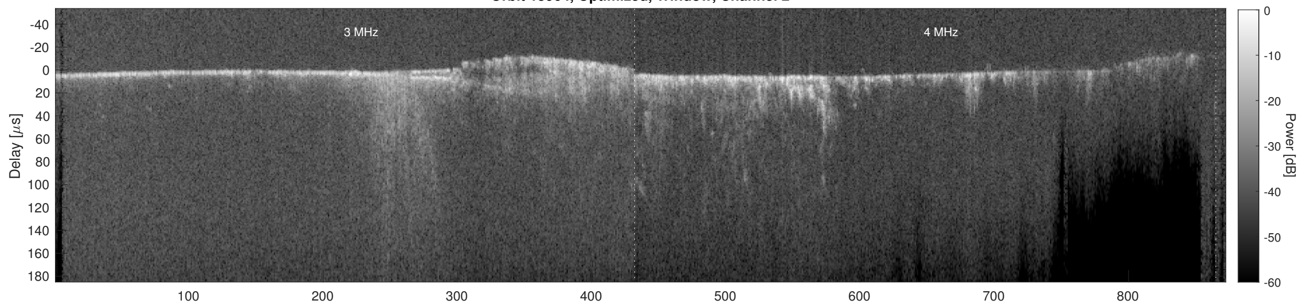
Orbit 15964, Cluttergram
