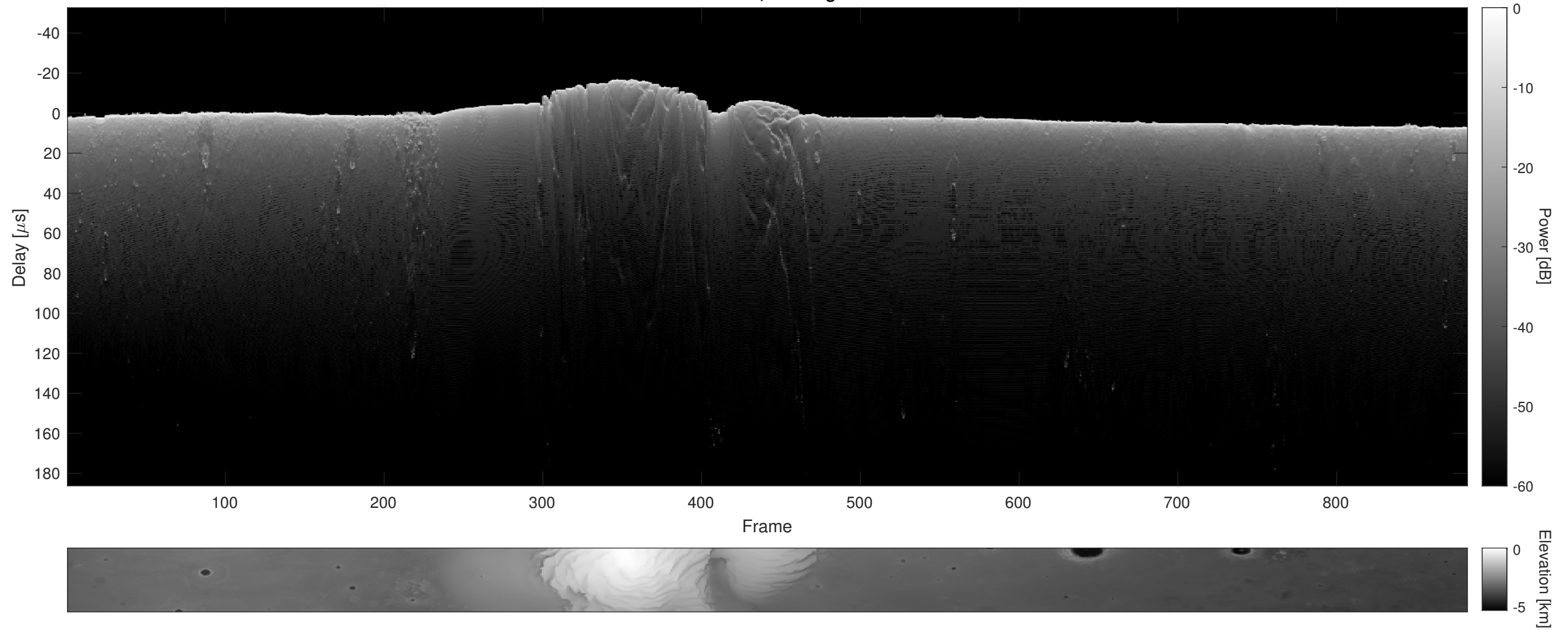
Orbit 15967, Cluttergram
