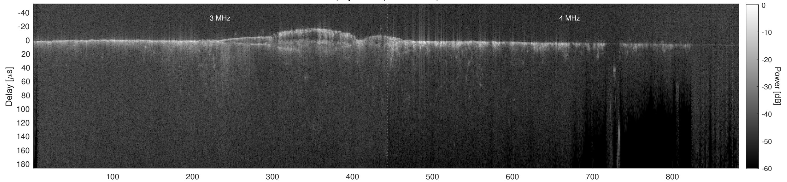
Orbit 15967, Cluttergram
