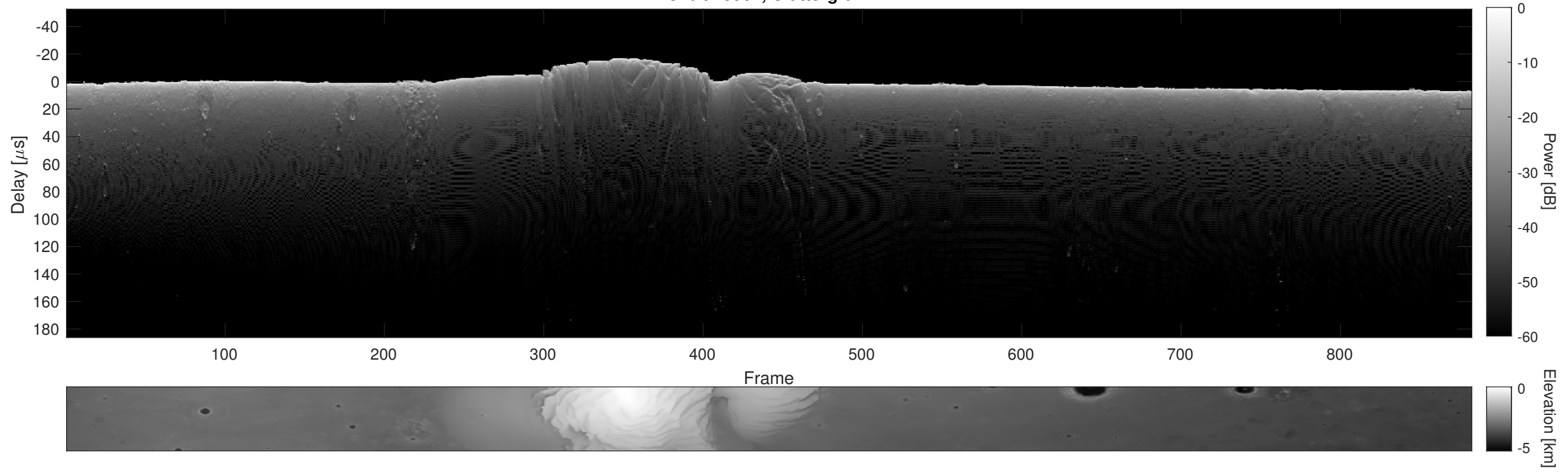
Orbit 15967, Cluttergram
