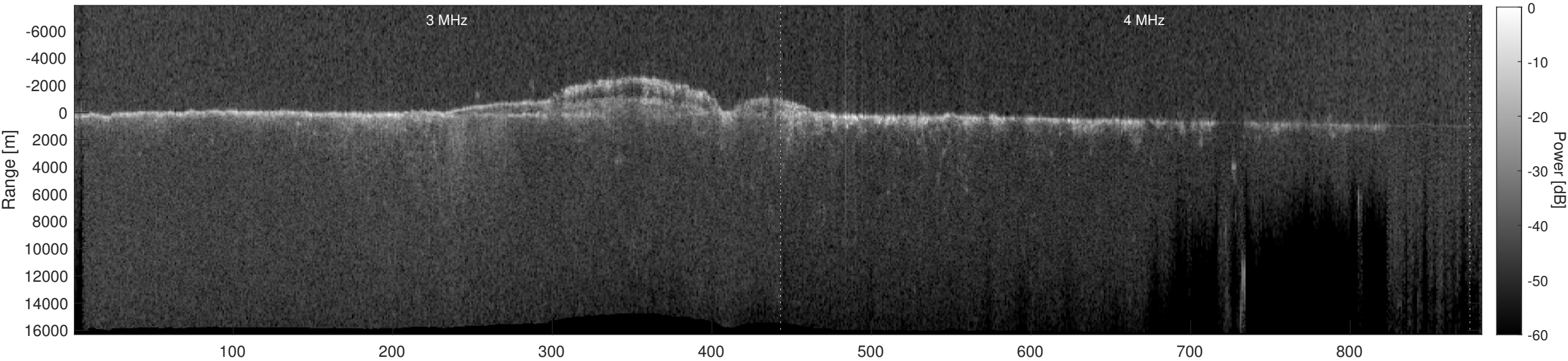
Orbit 15967, Depth-Corrected Cluttergram
