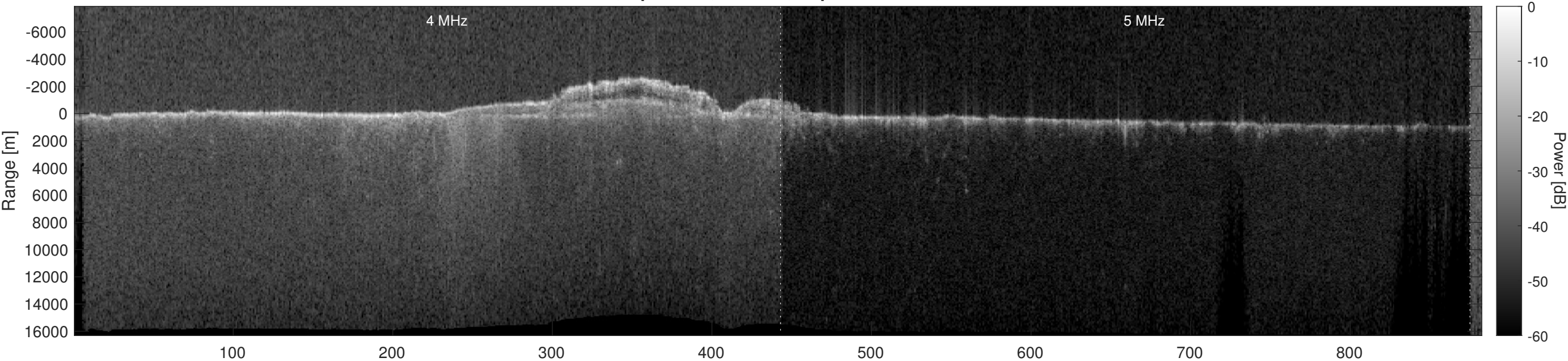
Orbit 15967, Optimized, Window, Depth-Corrected, Channel 2
