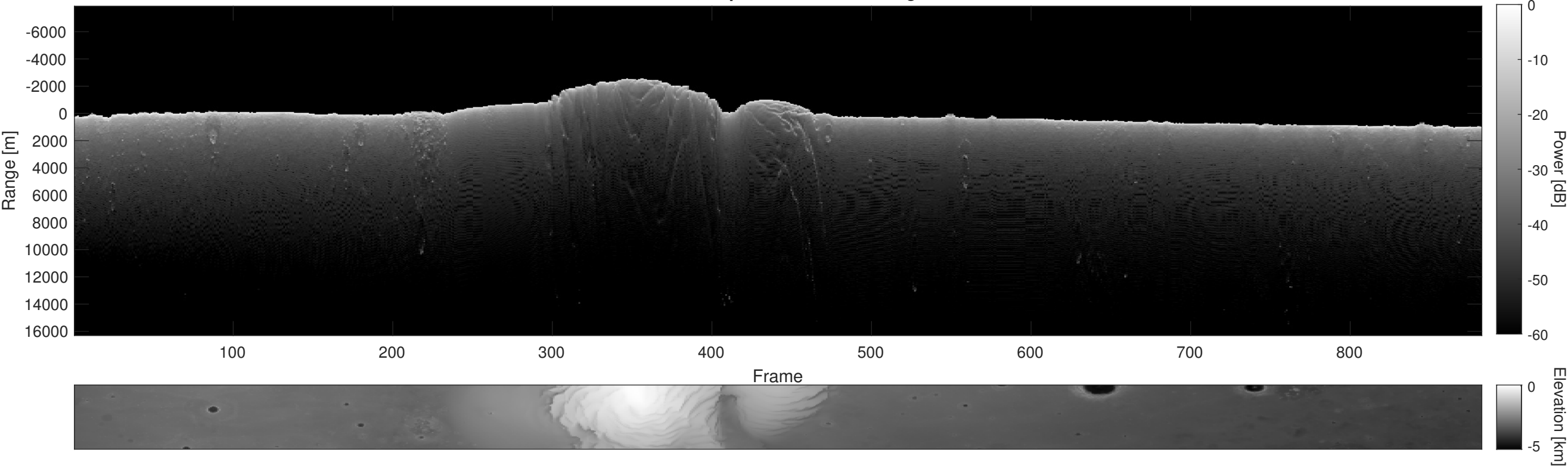
Orbit 15967, Depth-Corrected Cluttergram
