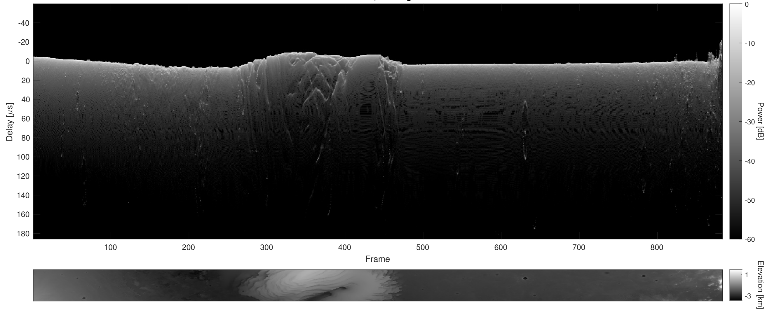
Orbit 15970, Cluttergram
