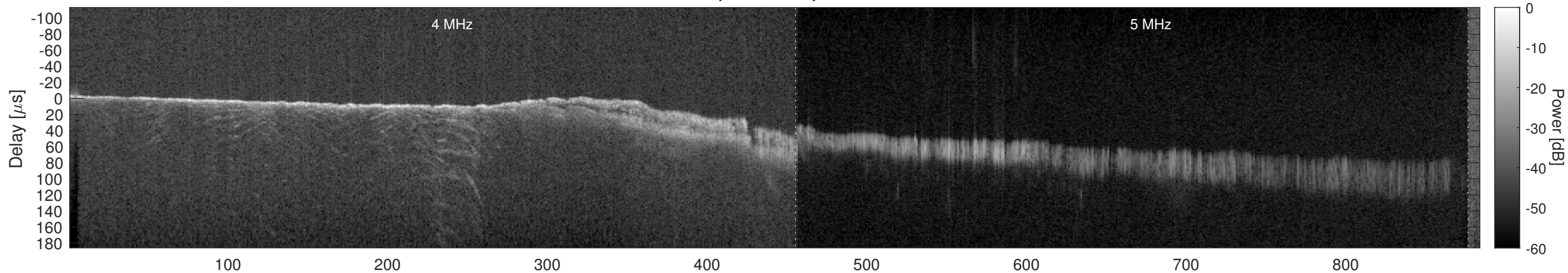
Orbit 15970, Window, Channel 1, Chapman
