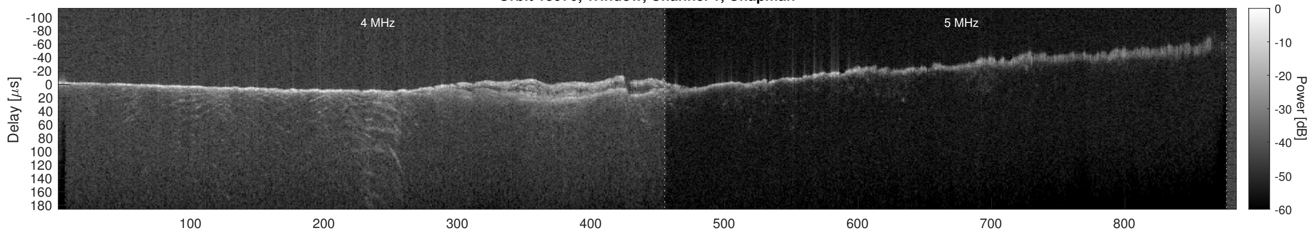
Orbit 15970, Window, Channel 1, Optimized
