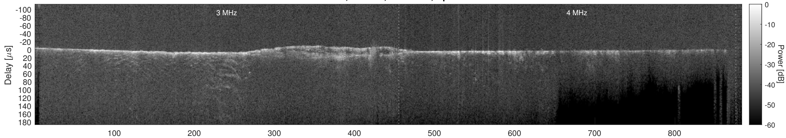
Orbit 15970, Cluttergram
