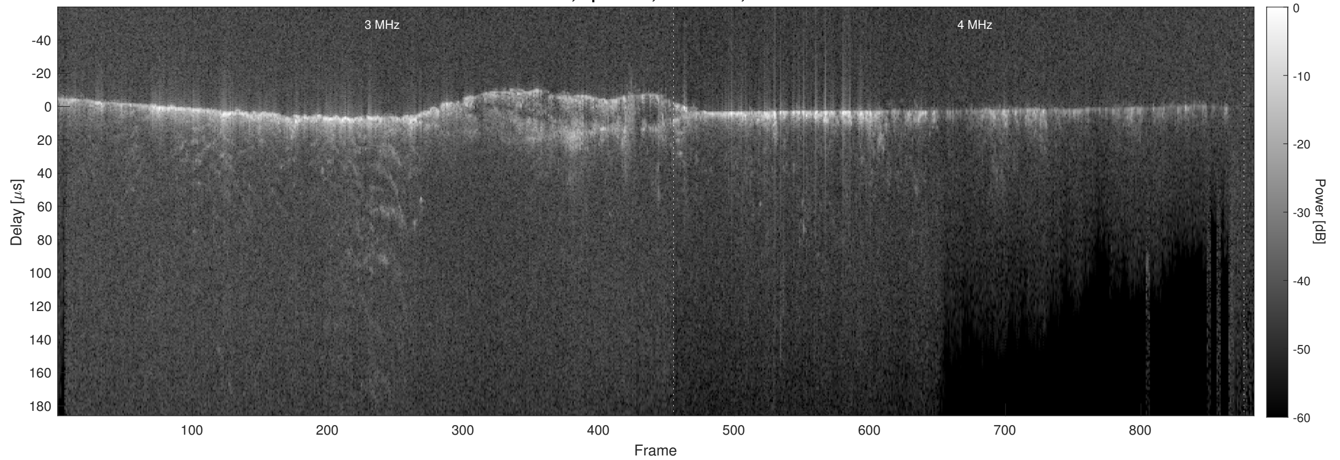
Orbit 15970, Optimized, No Window, Channel 2
