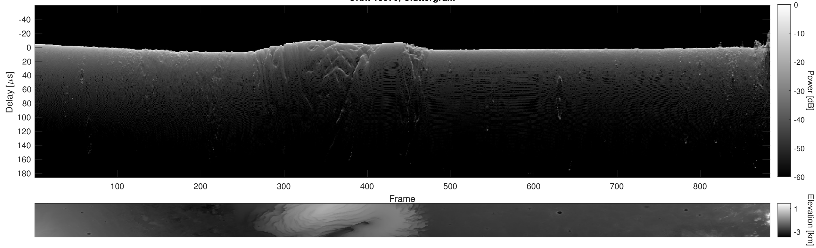
Orbit 15970, Cluttergram
