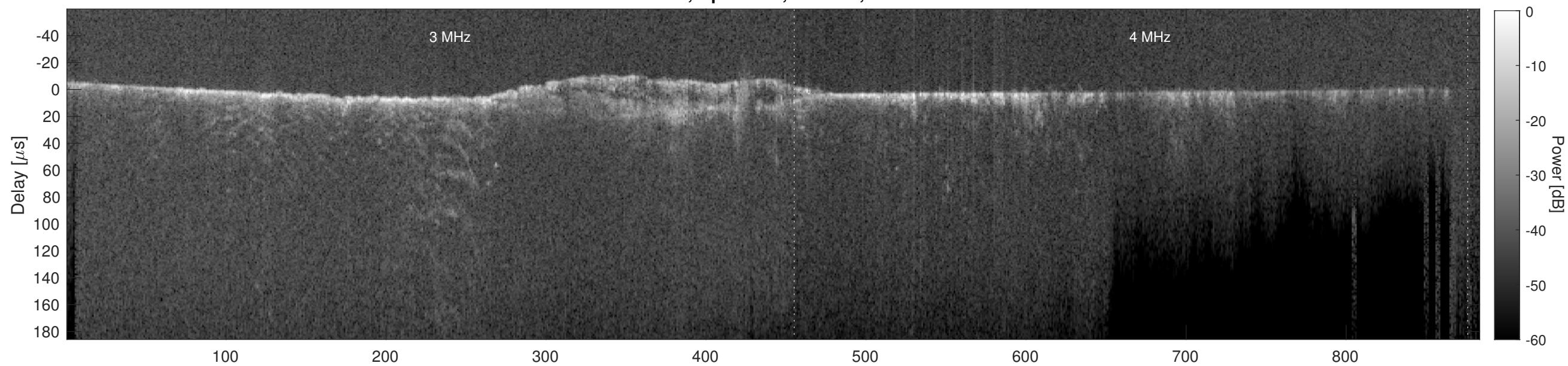
Orbit 15970, Cluttergram
