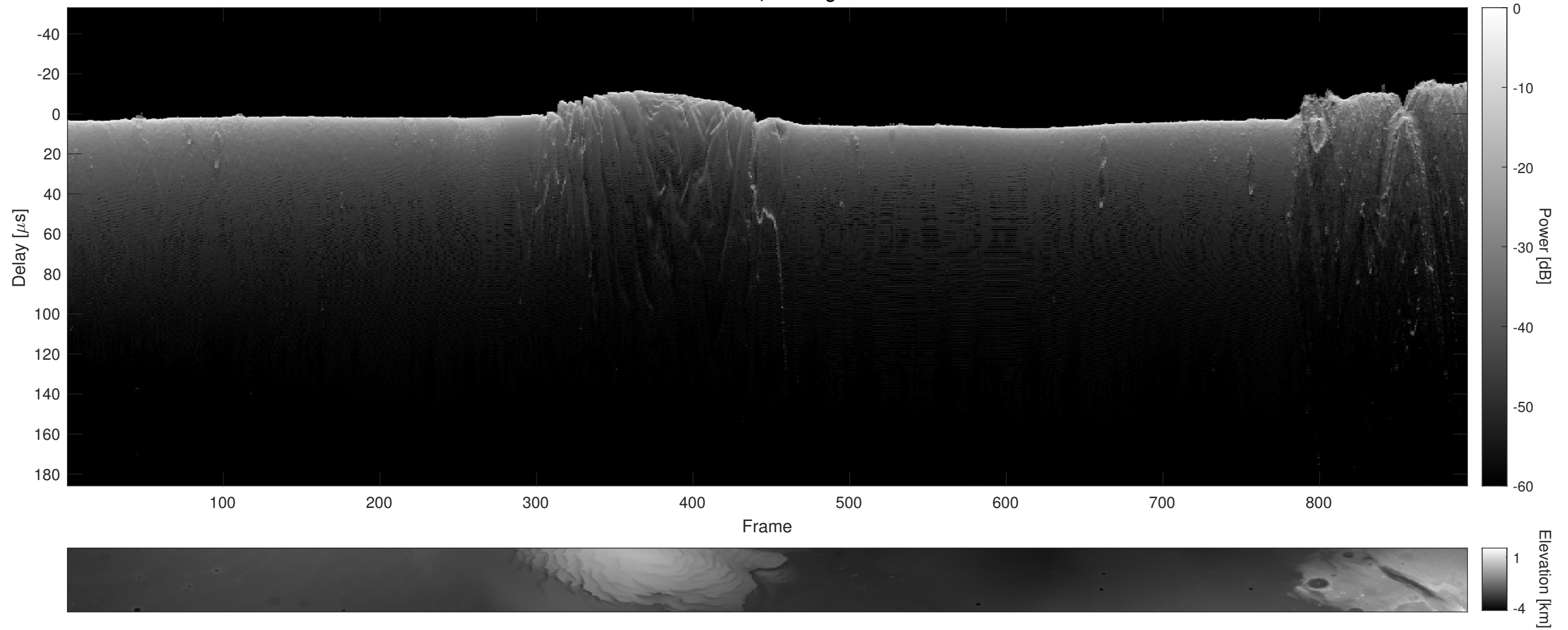
Orbit 15971, Cluttergram
