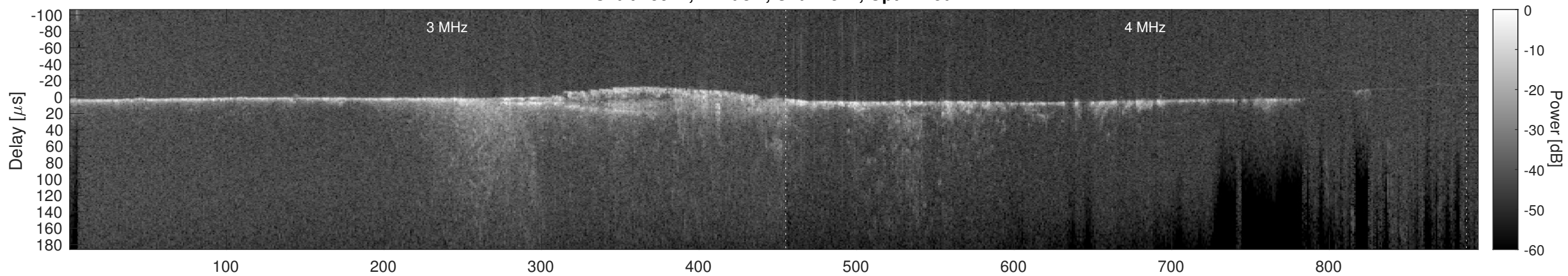
Orbit 15971, Cluttergram
