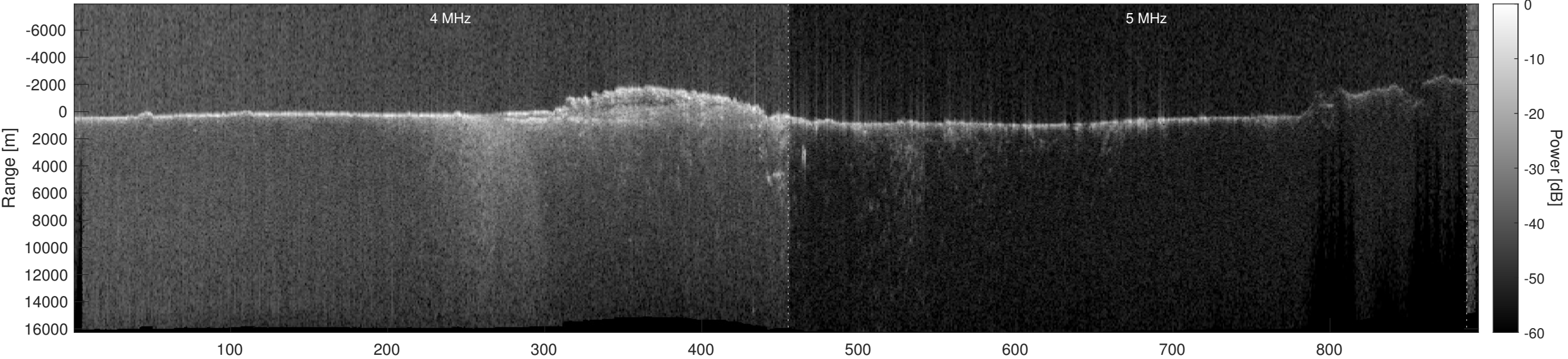
Orbit 15971, Optimized, Window, Depth-Corrected, Channel 2
