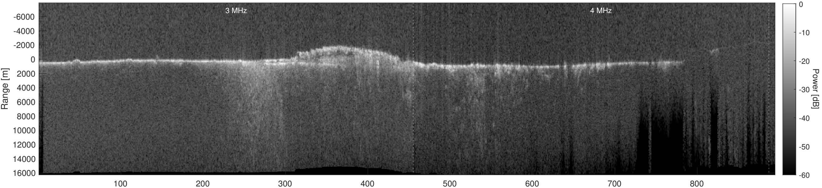
Orbit 15971, Depth-Corrected Cluttergram
