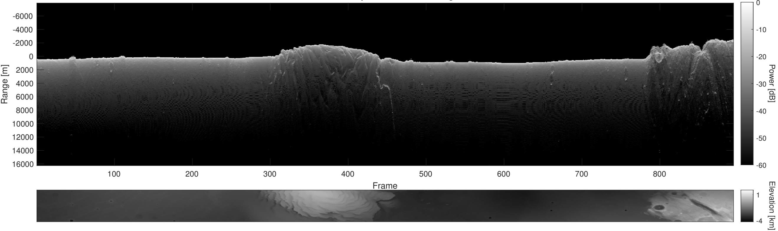
Orbit 15971, Depth-Corrected Cluttergram
