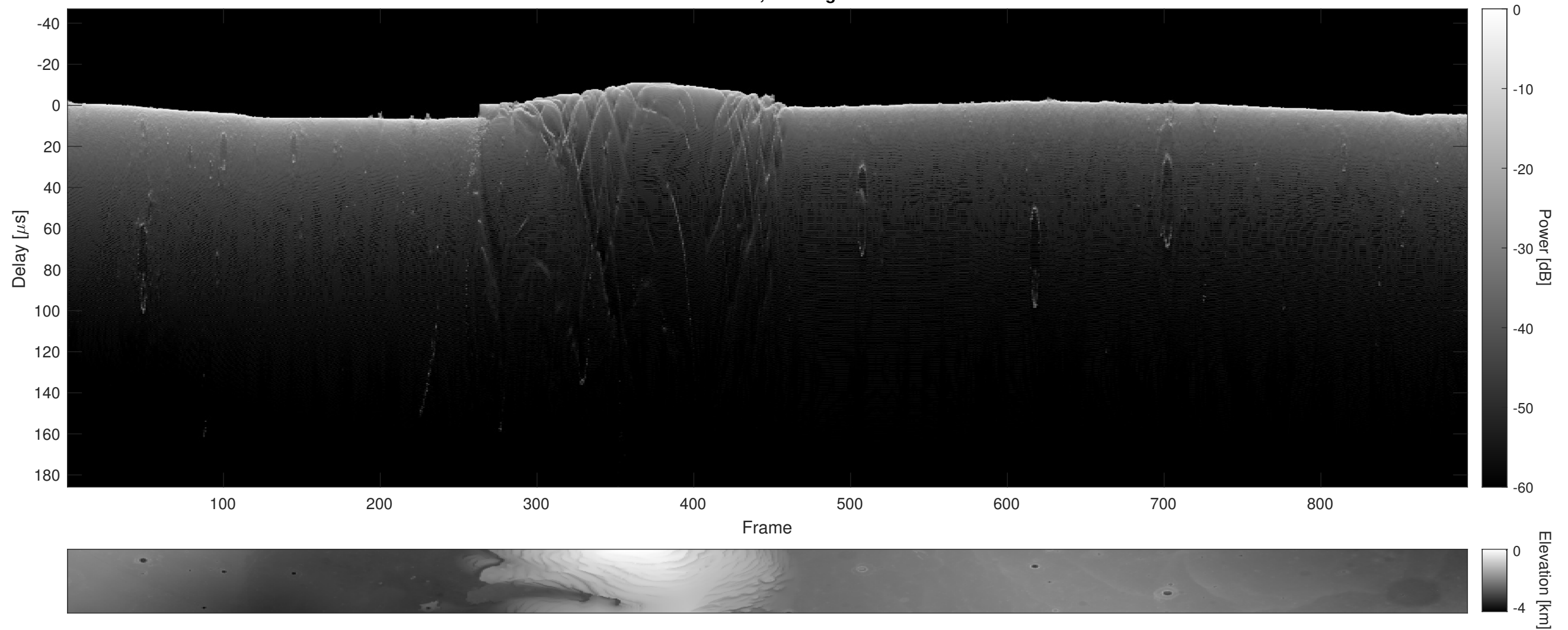
Orbit 15973, Cluttergram
