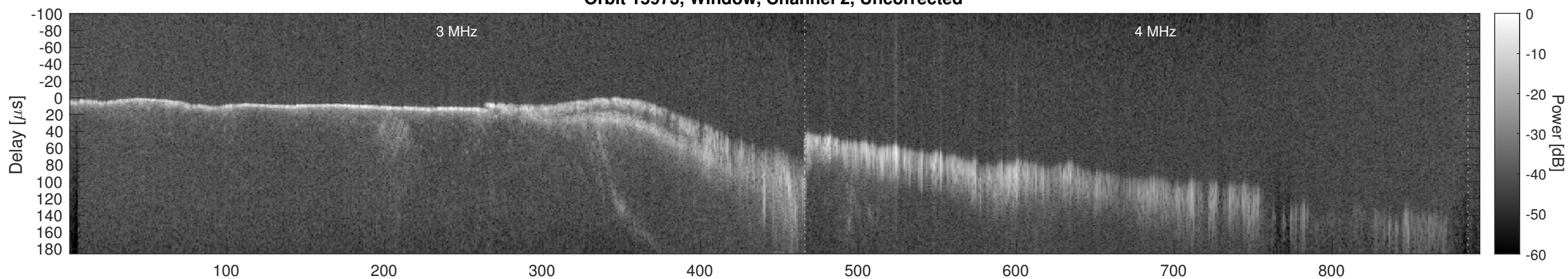
Orbit 15973, Window, Channel 2, Chapman
