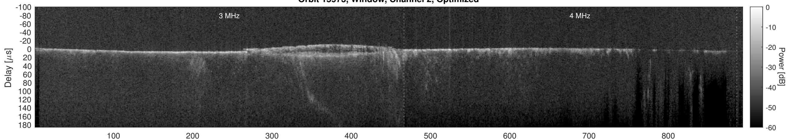
Orbit 15973, Cluttergram
