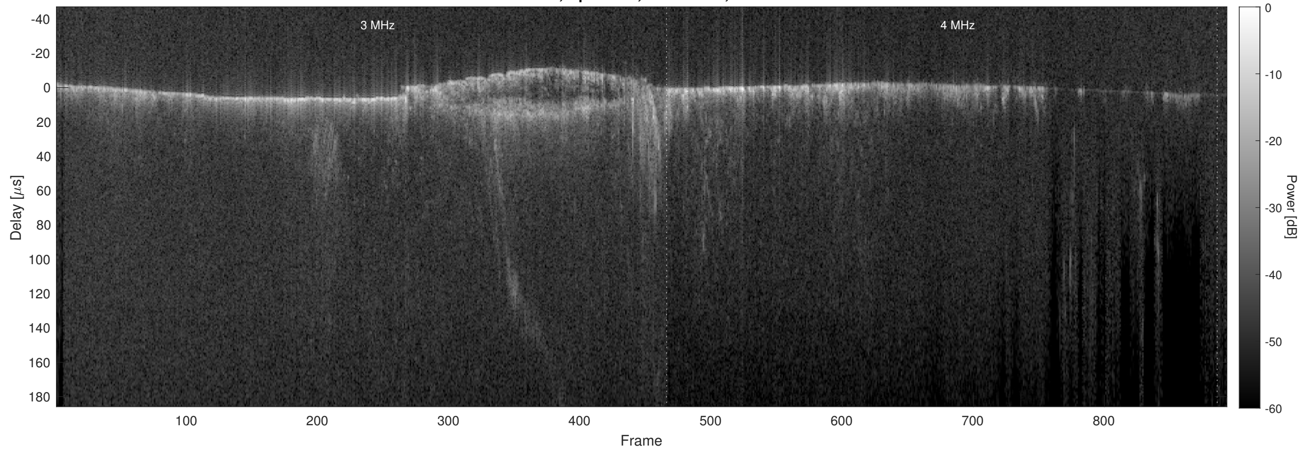
Orbit 15973, Optimized, No Window, Channel 2
