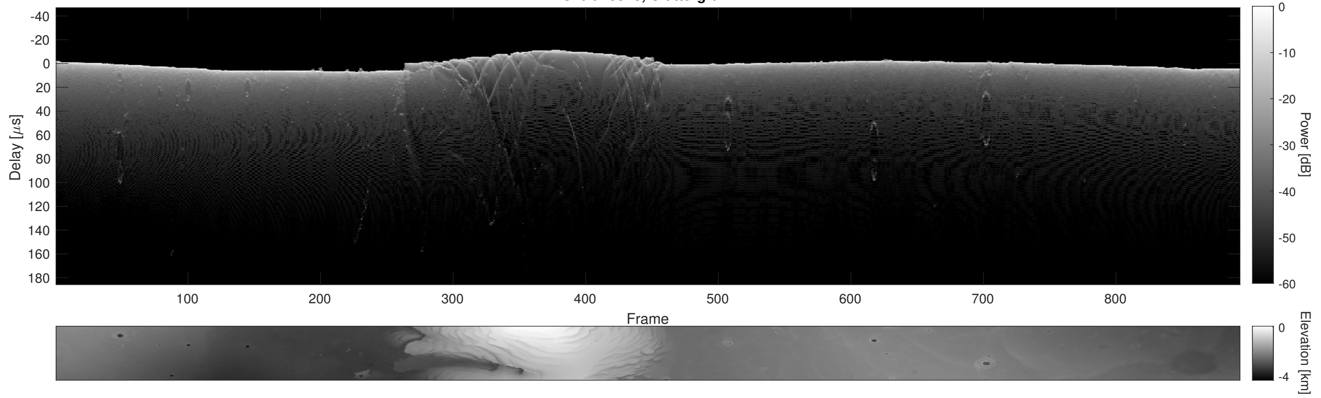
Orbit 15973, Cluttergram
