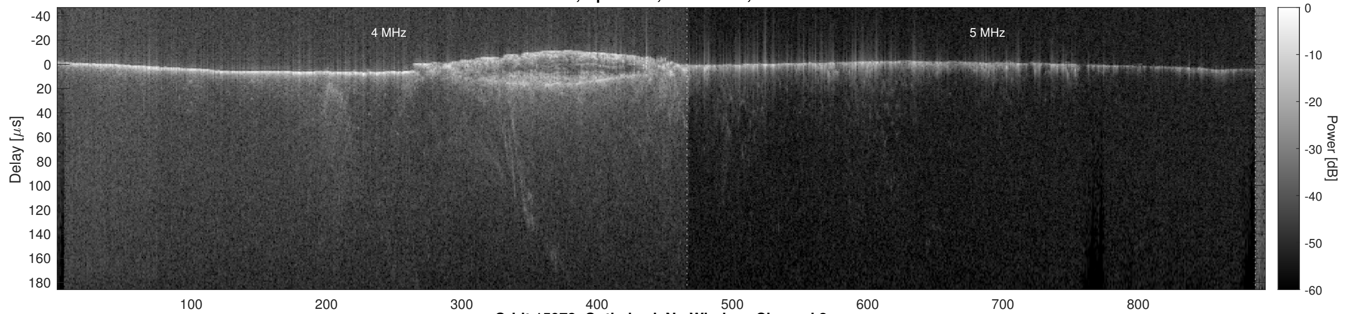
Orbit 15973, Optimized, No Window, Channel 2
