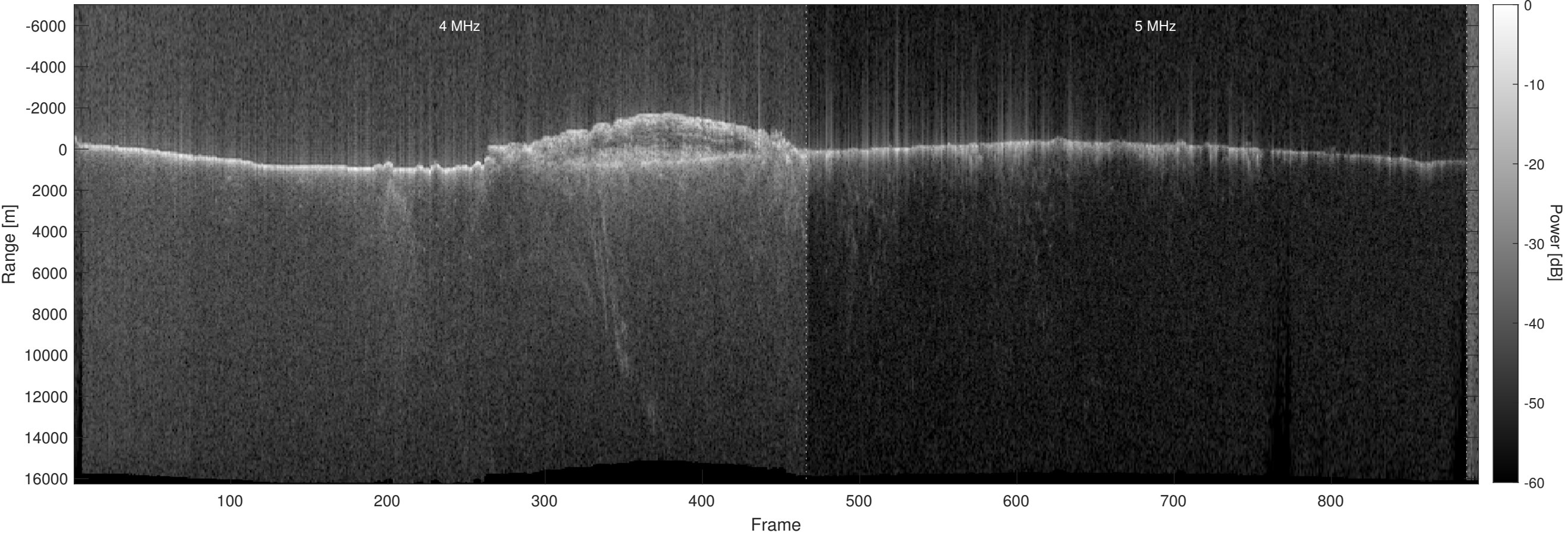
Orbit 15973, Optimized, No Window, Depth-Corrected, Channel 2
