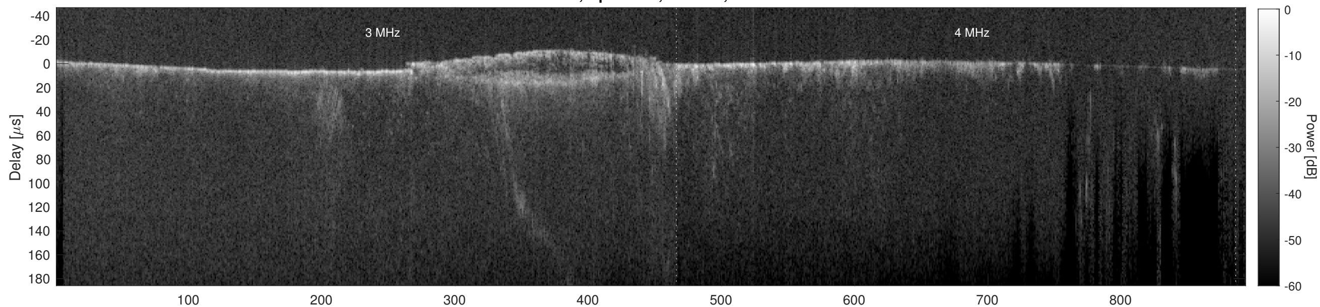
Orbit 15973, Cluttergram
