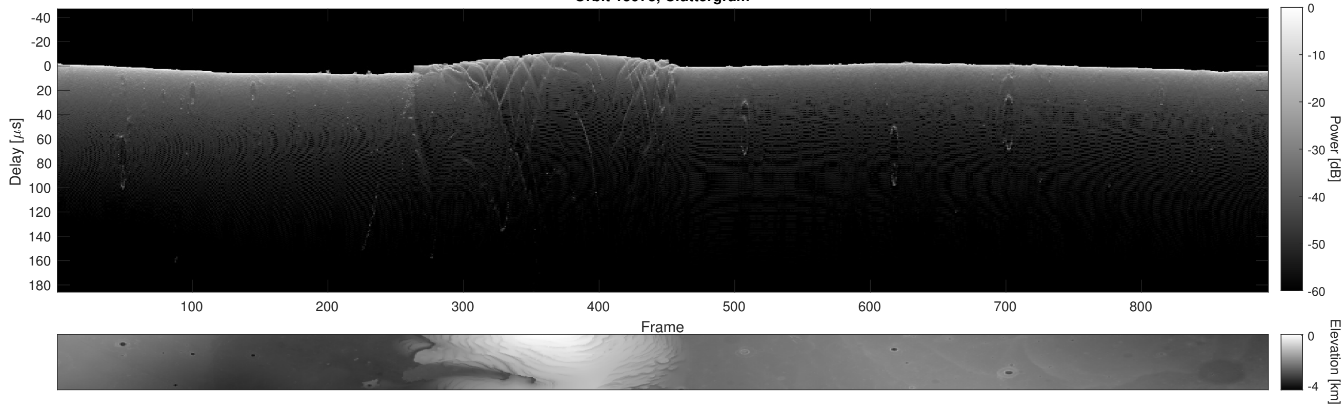
Orbit 15973, Cluttergram
