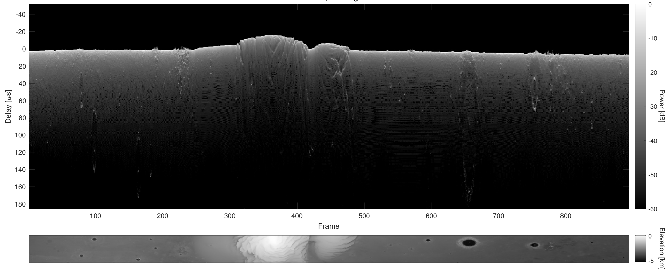
Orbit 15974, Cluttergram
