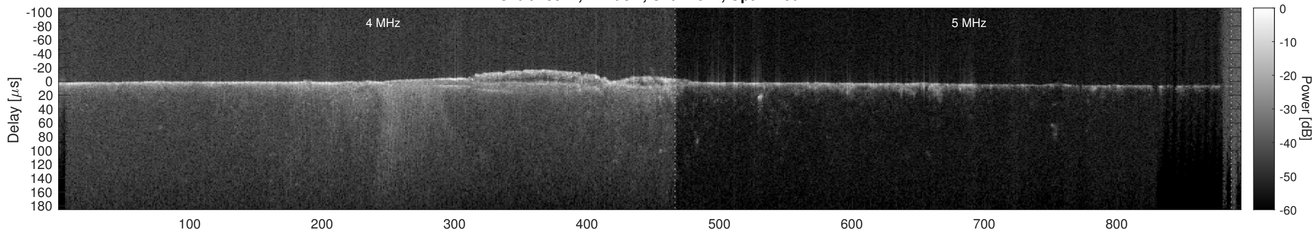
Orbit 15974, Cluttergram
