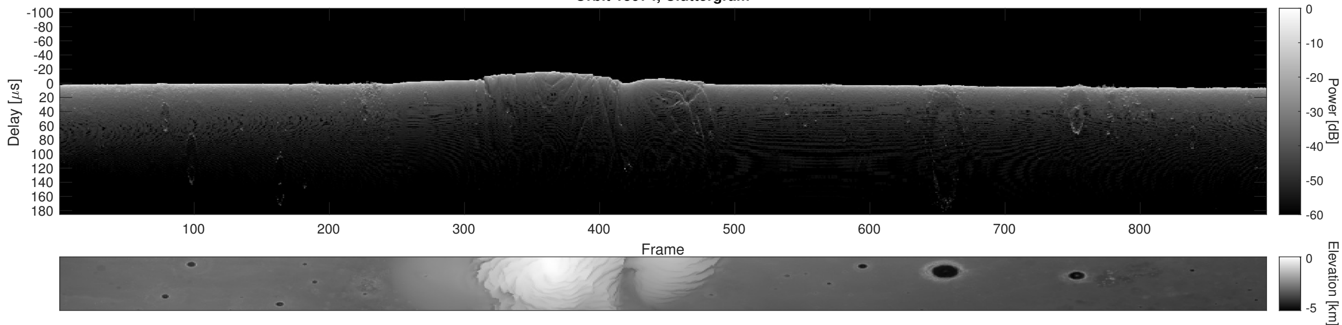
Orbit 15974, Cluttergram
