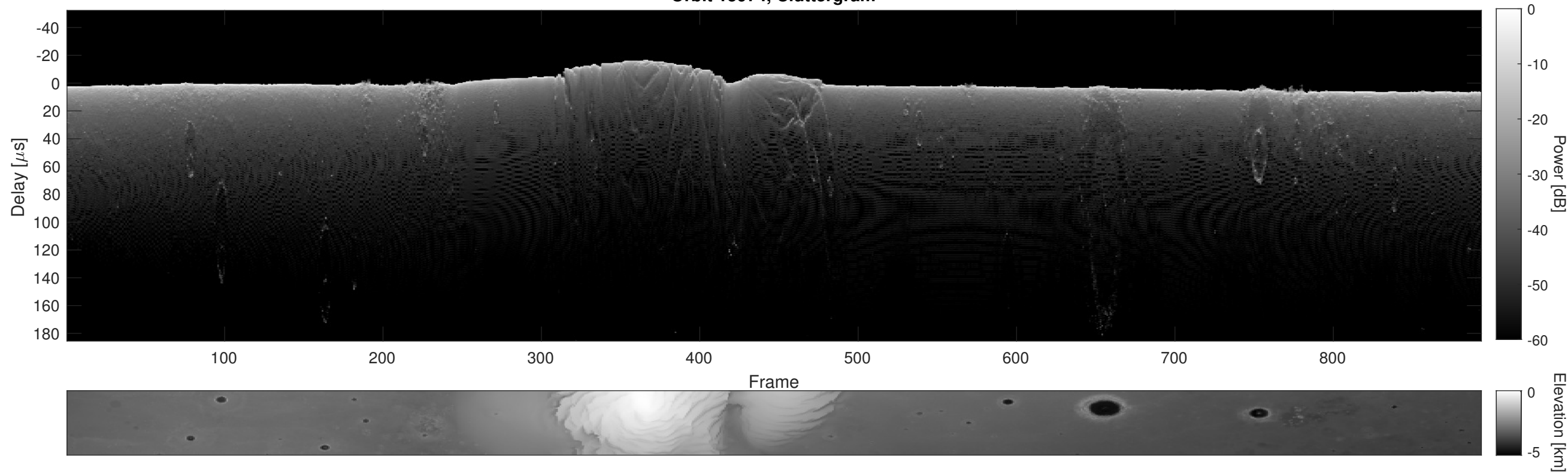
Orbit 15974, Cluttergram
