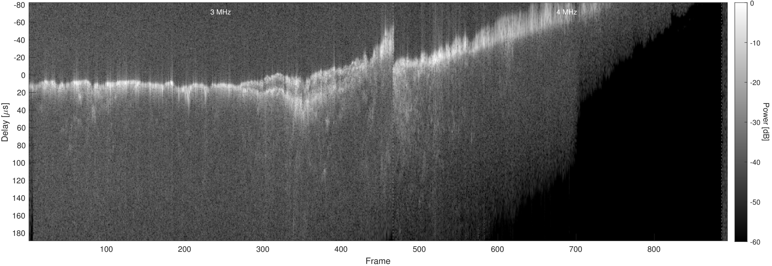
Orbit 15975, Chapman, No Window, Channel 2
