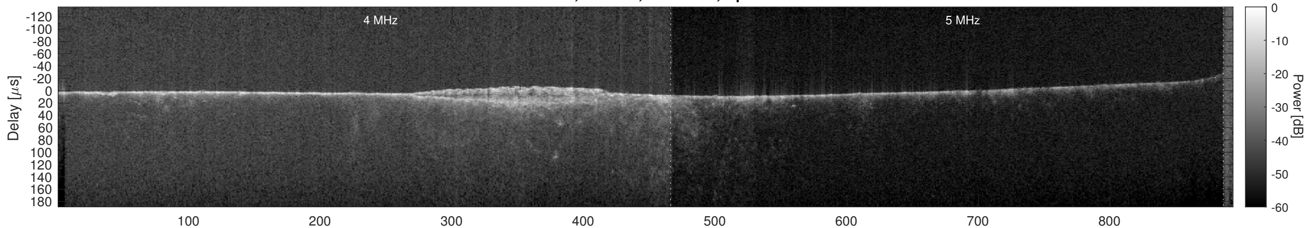
Orbit 15975, Cluttergram
