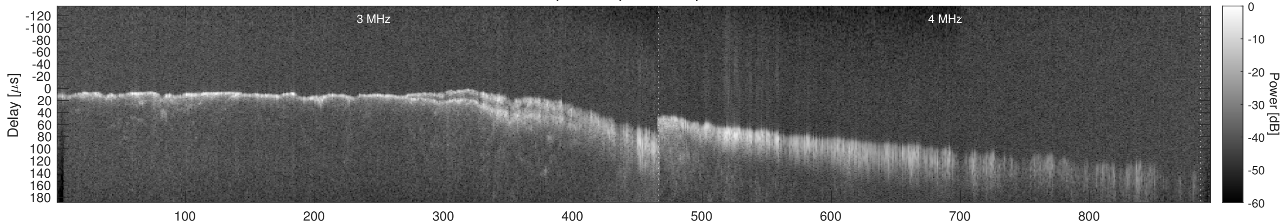
Orbit 15975, Window, Channel 2, Chapman
