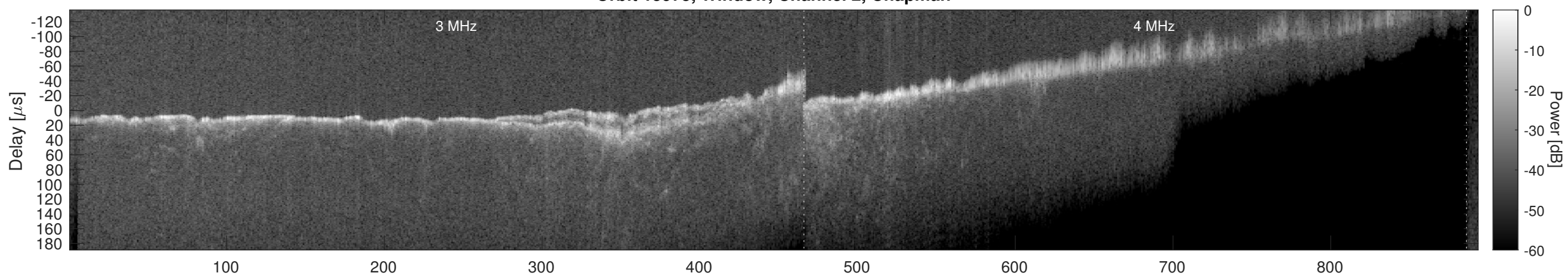
Orbit 15975, Window, Channel 2, Optimized
