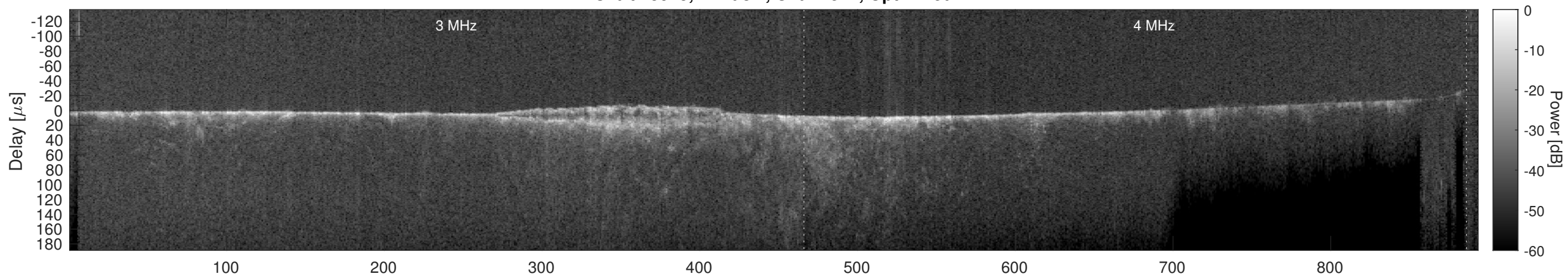
Orbit 15975, Cluttergram
