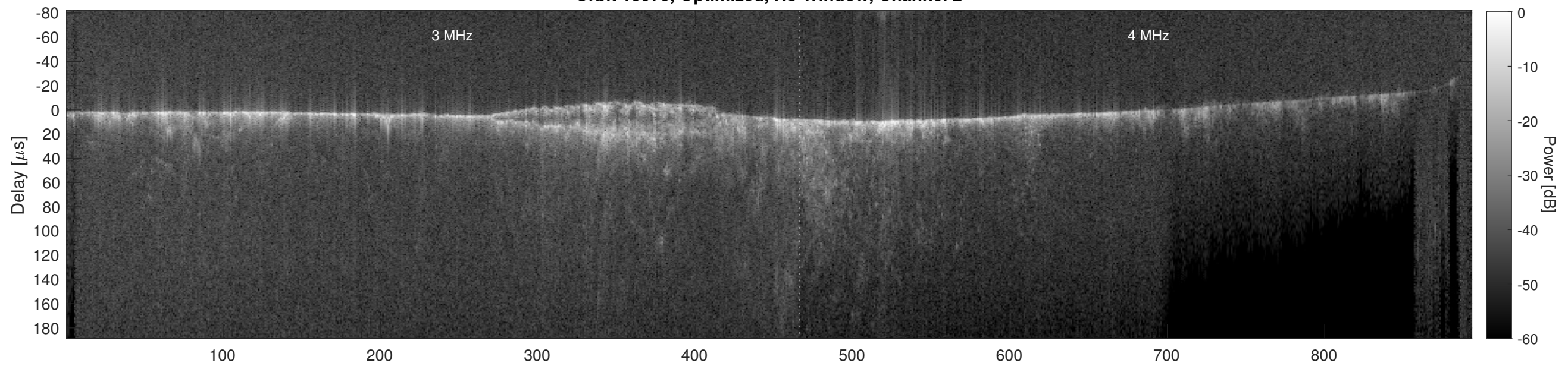
Orbit 15975, Cluttergram
