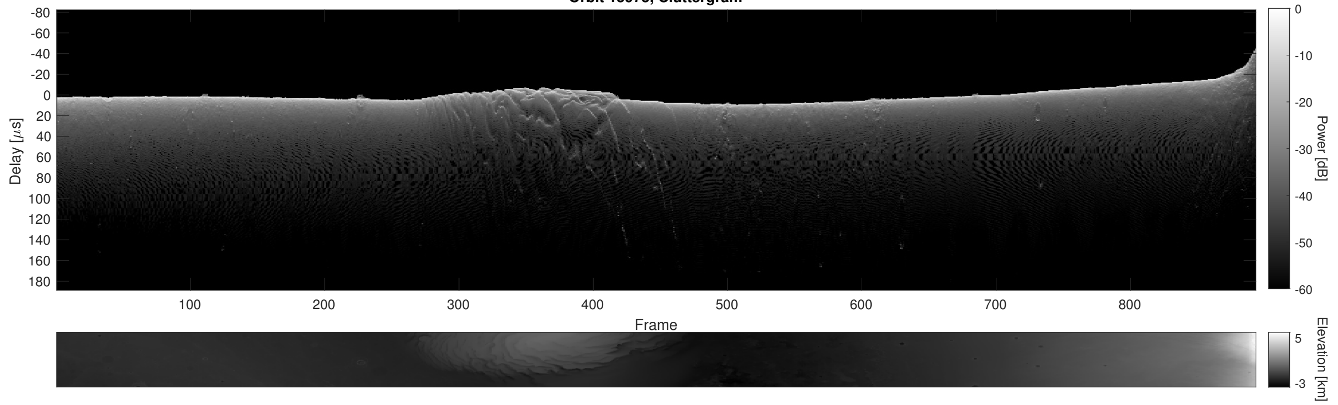
Orbit 15975, Cluttergram
