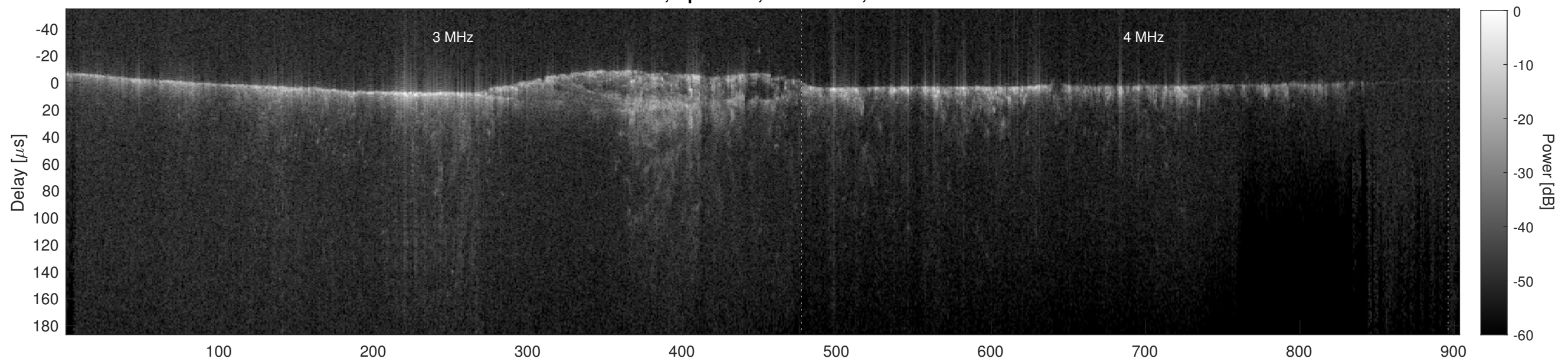
Orbit 15977, Cluttergram
