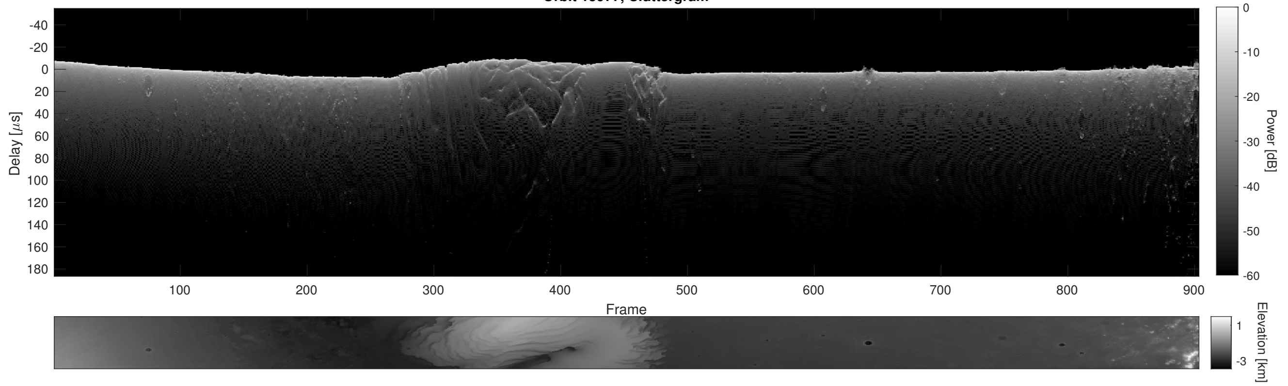
Orbit 15977, Cluttergram
