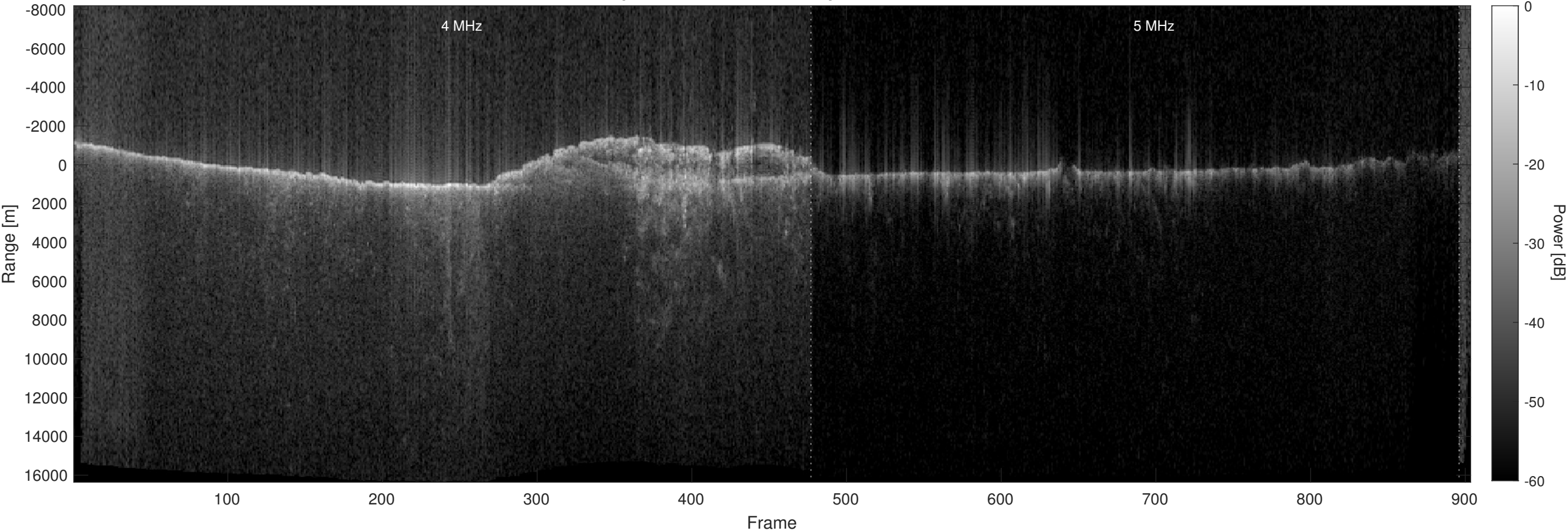
Orbit 15977, Optimized, No Window, Depth-Corrected, Channel 2
