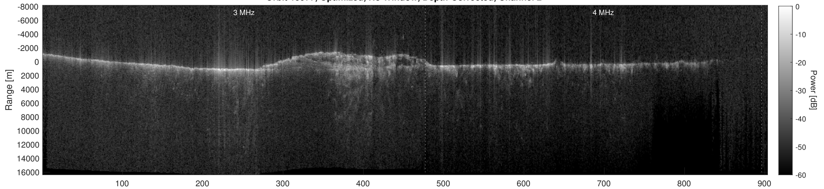
Orbit 15977, Depth-Corrected Cluttergram
