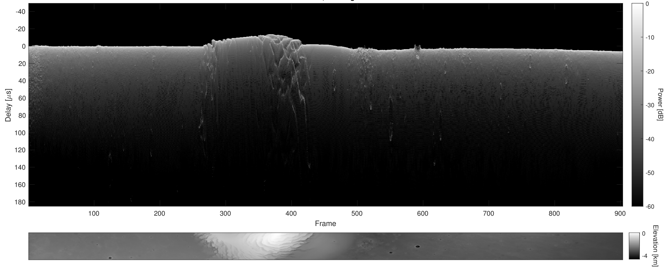
Orbit 15979, Cluttergram
