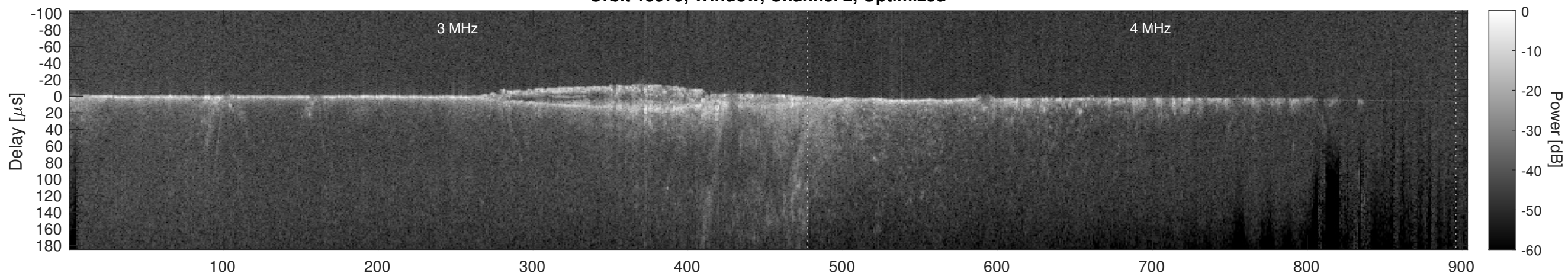
Orbit 15979, Cluttergram
