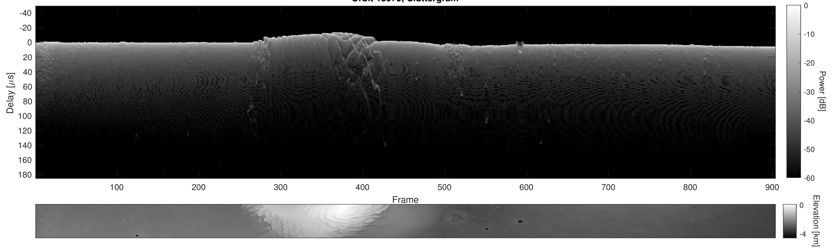
Orbit 15979, Cluttergram
