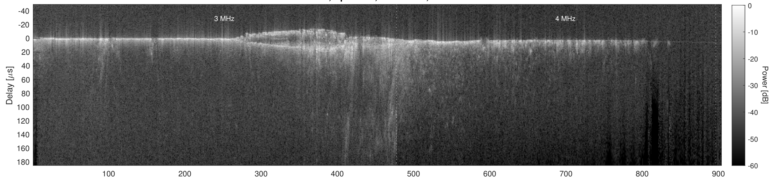
Orbit 15979, Cluttergram
