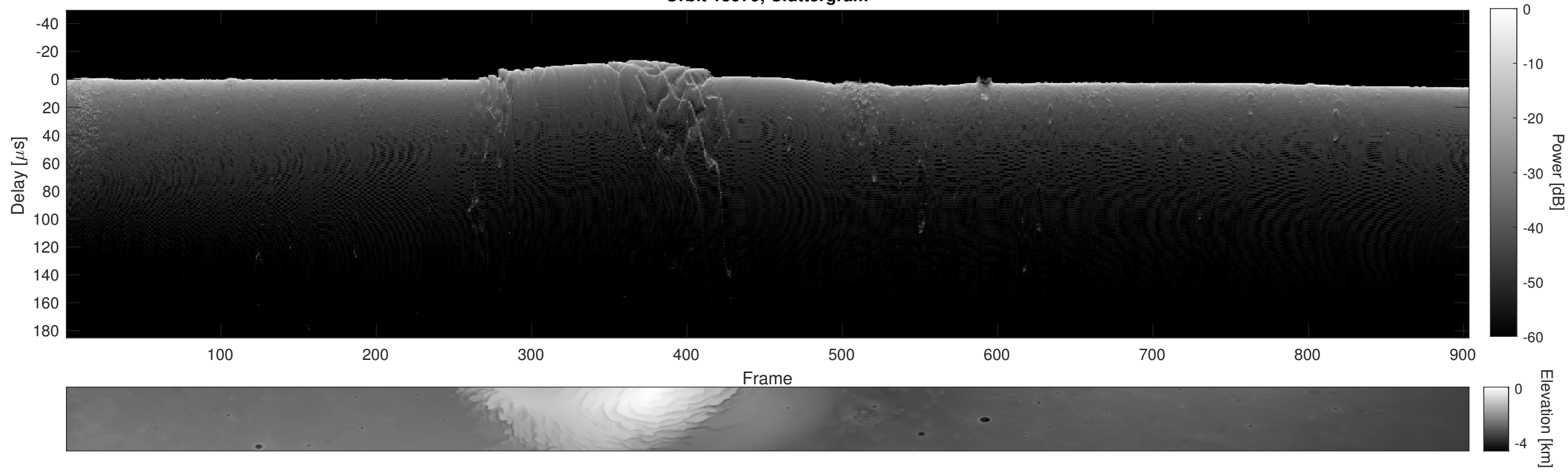
Orbit 15979, Cluttergram
