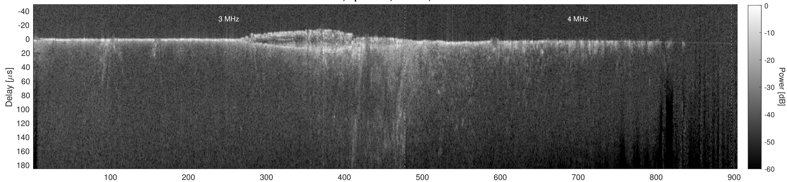
Orbit 15979, Cluttergram
