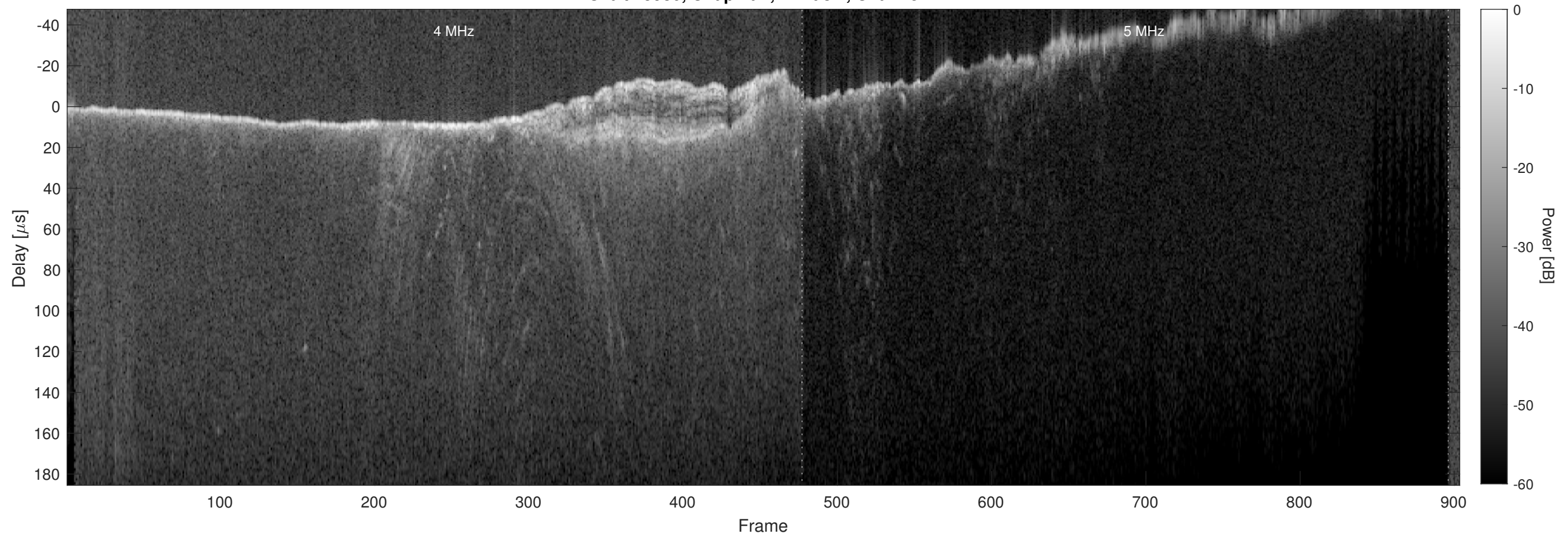
Orbit 15980, Chapman, Window, Channel 2
