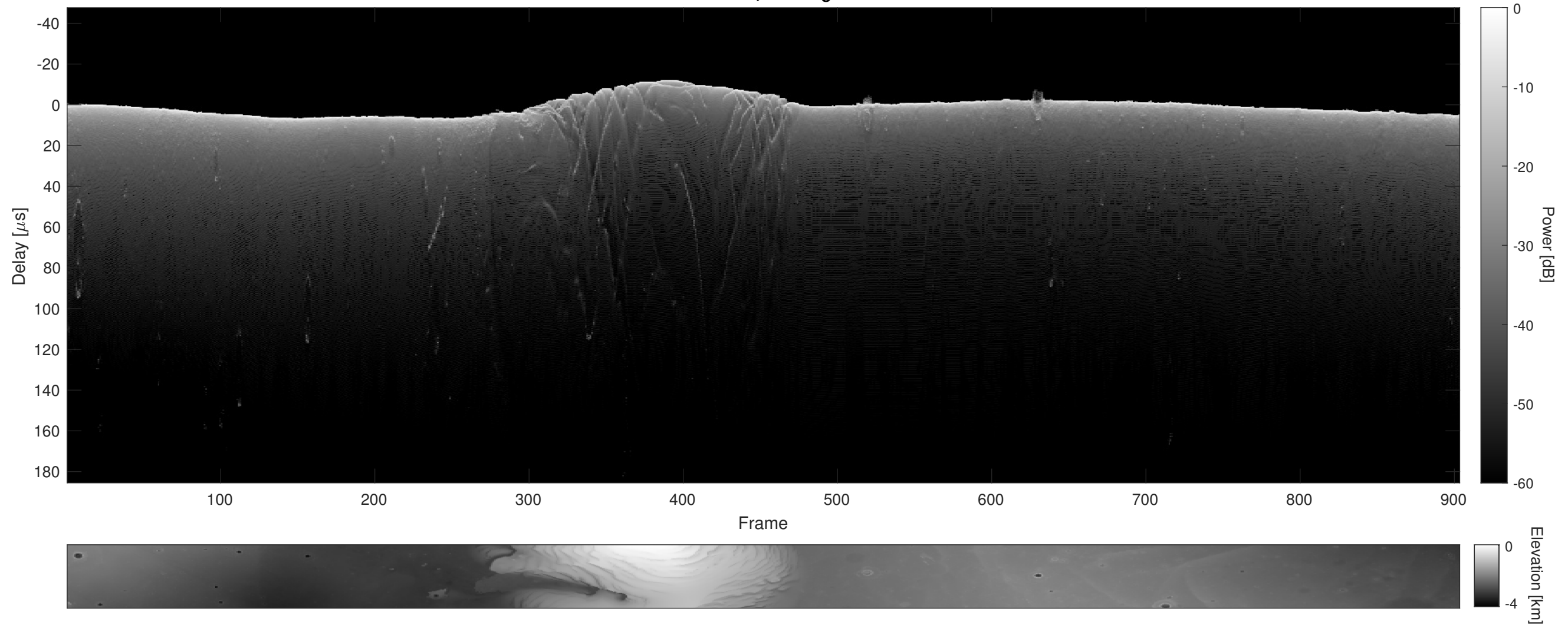
Orbit 15980, Cluttergram
