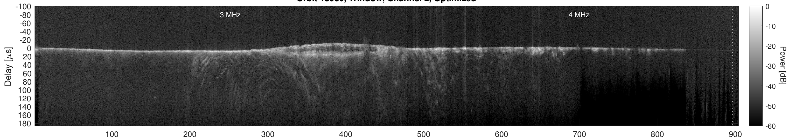
Orbit 15980, Cluttergram
